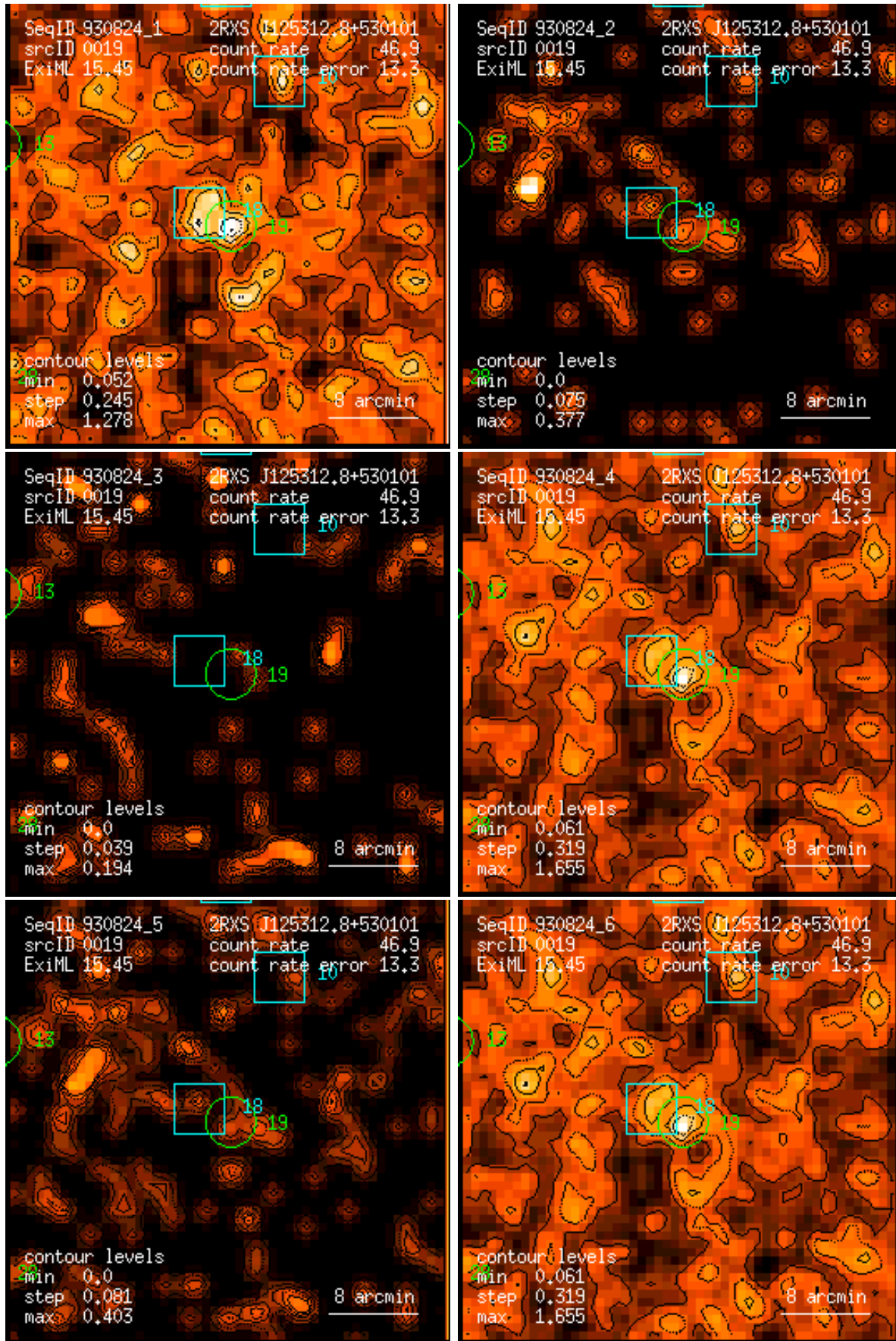
Figure 19: RASS 930824: detection 0019: band rate images, Gaussian filter: (1) PSPC channels 11 – 41, (2) 52 – 90, (3) 91 – 201, (4) 11 – 235, (5) 52 – 201, (6) 11 – 201. Broad band rates in counts/ks. Band rate contour levels in counts/ks/arcmin 2 .
