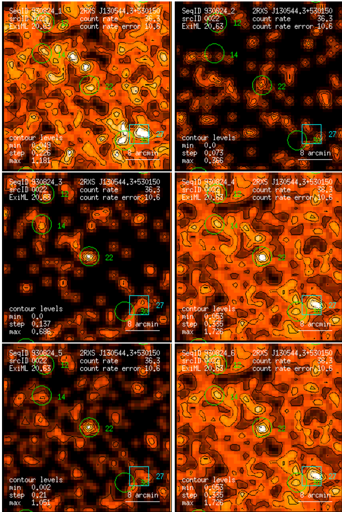
Figure 22: RASS 930824: detection 0022: band rate images, Gaussian filter: (1) PSPC channels 11 – 41, (2) 52 – 90, (3) 91 – 201, (4) 11 – 235, (5) 52 – 201, (6) 11 – 201. Broad band rates in counts/ks. Band rate contour levels in counts/ks/arcmin 2 .
