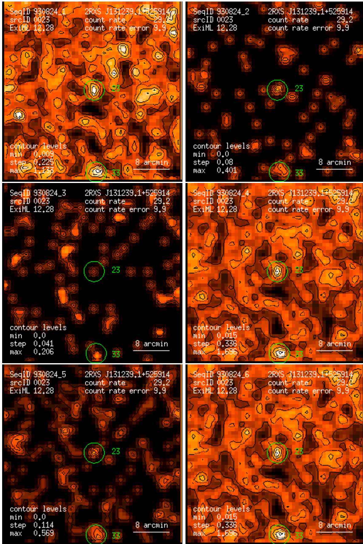
Figure 23: RASS 930824: detection 0023: band rate images, Gaussian filter: (1) PSPC channels 11 – 41, (2) 52 – 90, (3) 91 – 201, (4) 11 – 235, (5) 52 – 201, (6) 11 – 201. Broad band rates in counts/ks. Band rate contour levels in counts/ks/arcmin 2 .
