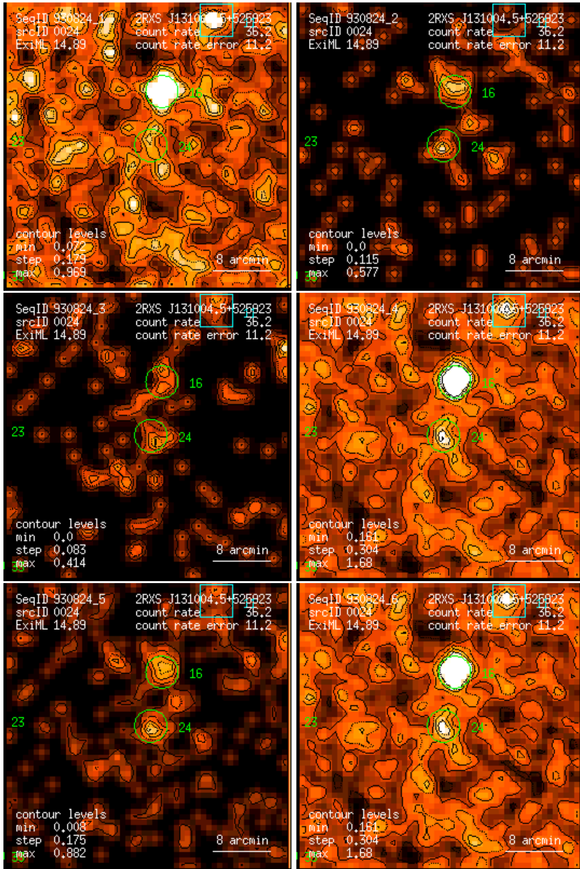
Figure 24: RASS 930824: detection 0024: band rate images, Gaussian filter: (1) PSPC channels 11 – 41, (2) 52 – 90, (3) 91 – 201, (4) 11 – 235, (5) 52 – 201, (6) 11 – 201. Broad band rates in counts/ks. Band rate contour levels in counts/ks/arcmin 2 .
