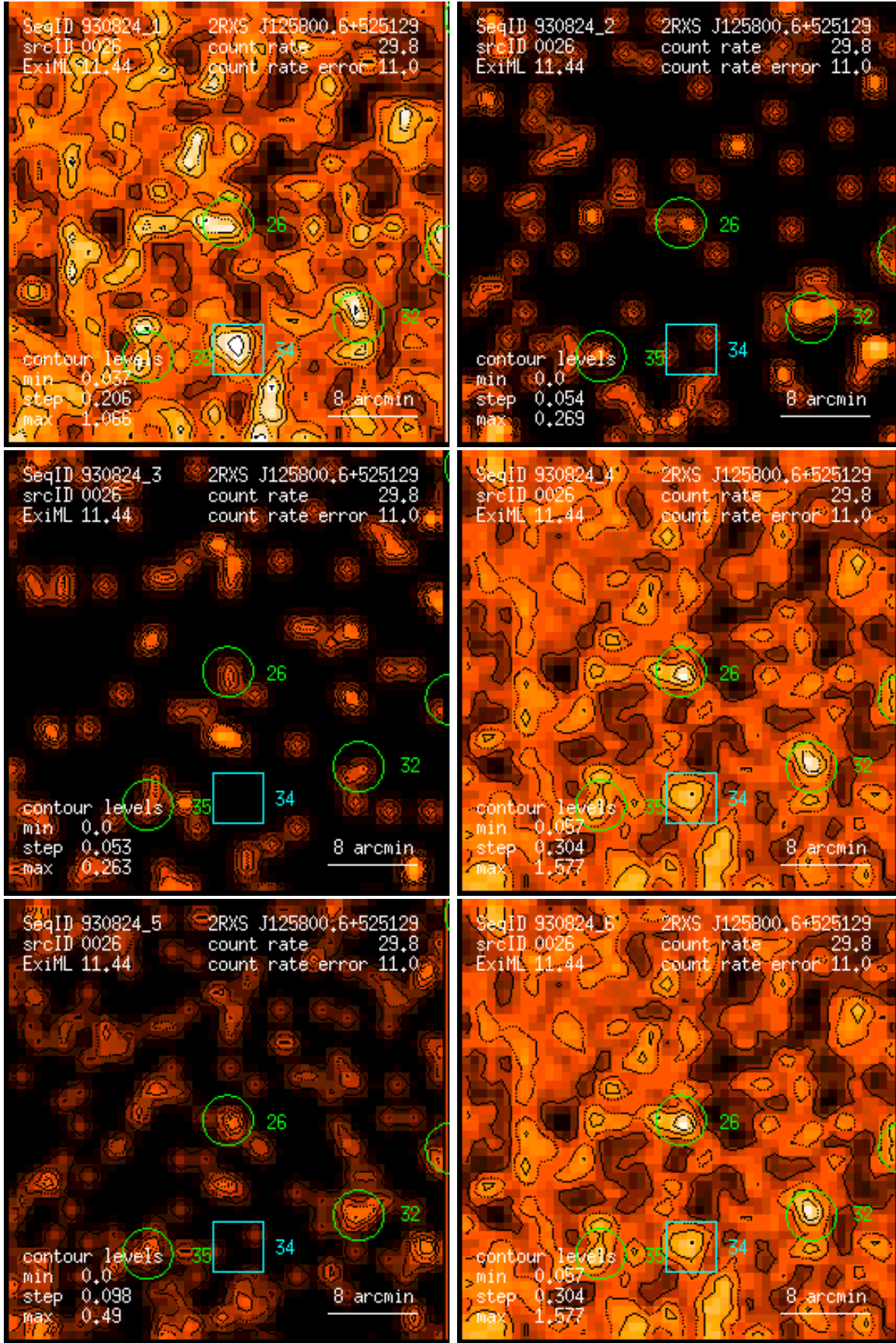
Figure 26: RASS 930824: detection 0026: band rate images, Gaussian filter: (1) PSPC channels 11 – 41, (2) 52 – 90, (3) 91 – 201, (4) 11 – 235, (5) 52 – 201, (6) 11 – 201. Broad band rates in counts/ks. Band rate contour levels in counts/ks/arcmin 2 .
