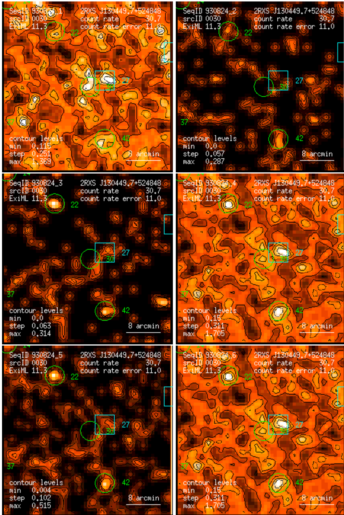
Figure 30: RASS 930824: detection 0030: band rate images, Gaussian filter: (1) PSPC channels 11 – 41, (2) 52 – 90, (3) 91 – 201, (4) 11 – 235, (5) 52 – 201, (6) 11 – 201. Broad band rates in counts/ks. Band rate contour levels in counts/ks/arcmin 2 .
