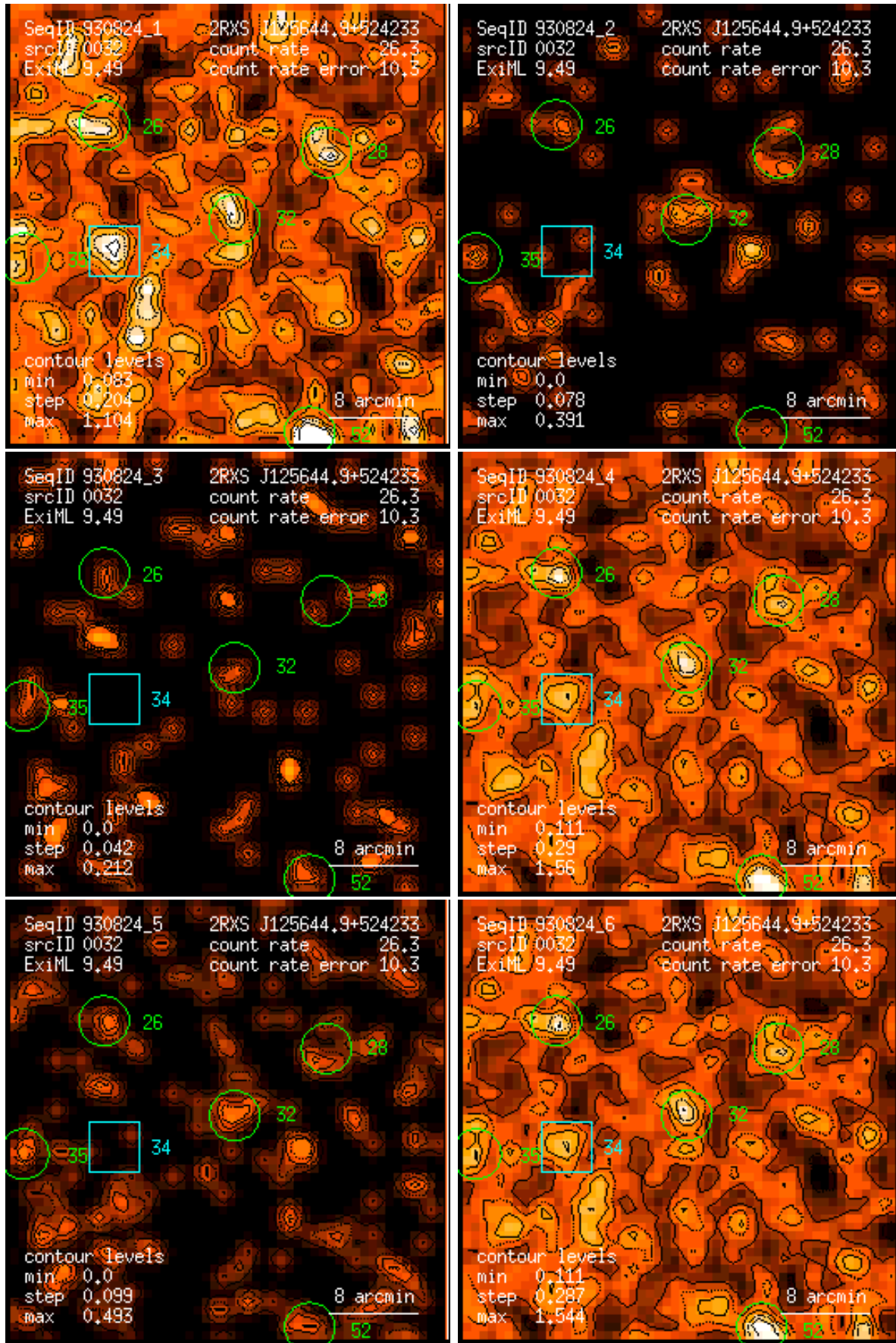
Figure 32: RASS 930824: detection 0032: band rate images, Gaussian filter: (1) PSPC channels 11 – 41, (2) 52 – 90, (3) 91 – 201, (4) 11 – 235, (5) 52 – 201, (6) 11 – 201. Broad band rates in counts/ks. Band rate contour levels in counts/ks/arcmin 2 .
