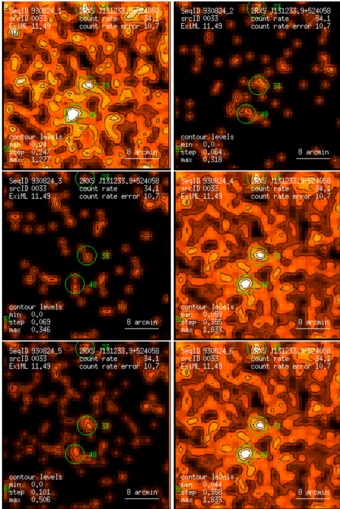
Figure 33: RASS 930824: detection 0033: band rate images, Gaussian filter: (1) PSPC channels 11 – 41, (2) 52 – 90, (3) 91 – 201, (4) 11 – 235, (5) 52 – 201, (6) 11 – 201. Broad band rates in counts/ks. Band rate contour levels in counts/ks/arcmin 2 .
