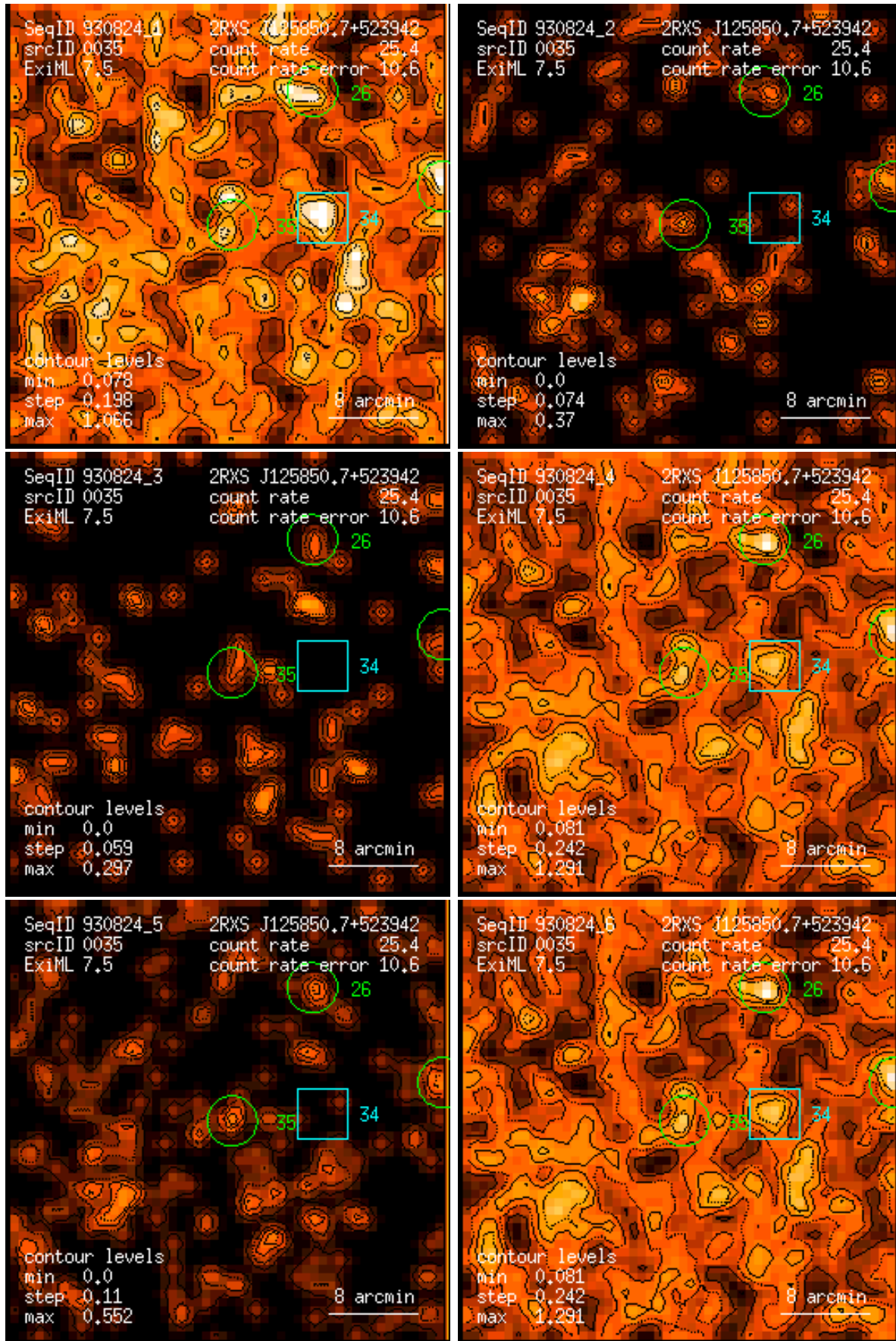
Figure 35: RASS 930824: detection 0035: band rate images, Gaussian filter: (1) PSPC channels 11 – 41, (2) 52 – 90, (3) 91 – 201, (4) 11 – 235, (5) 52 – 201, (6) 11 – 201. Broad band rates in counts/ks. Band rate contour levels in counts/ks/arcmin 2 .
