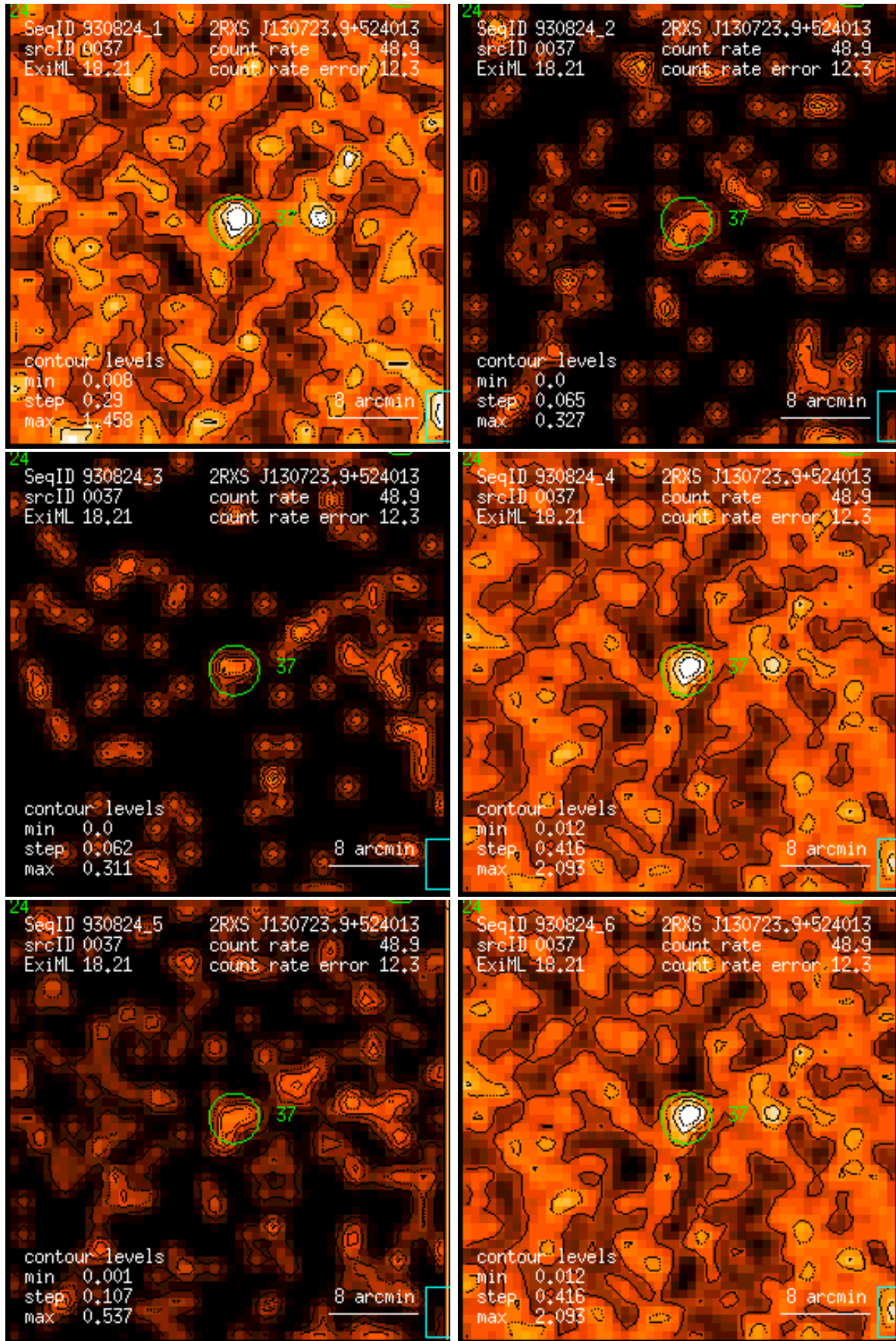
Figure 37: RASS 930824: detection 0037: band rate images, Gaussian filter: (1) PSPC channels 11 – 41, (2) 52 – 90, (3) 91 – 201, (4) 11 – 235, (5) 52 – 201, (6) 11 – 201. Broad band rates in counts/ks. Band rate contour levels in counts/ks/arcmin 2 .
