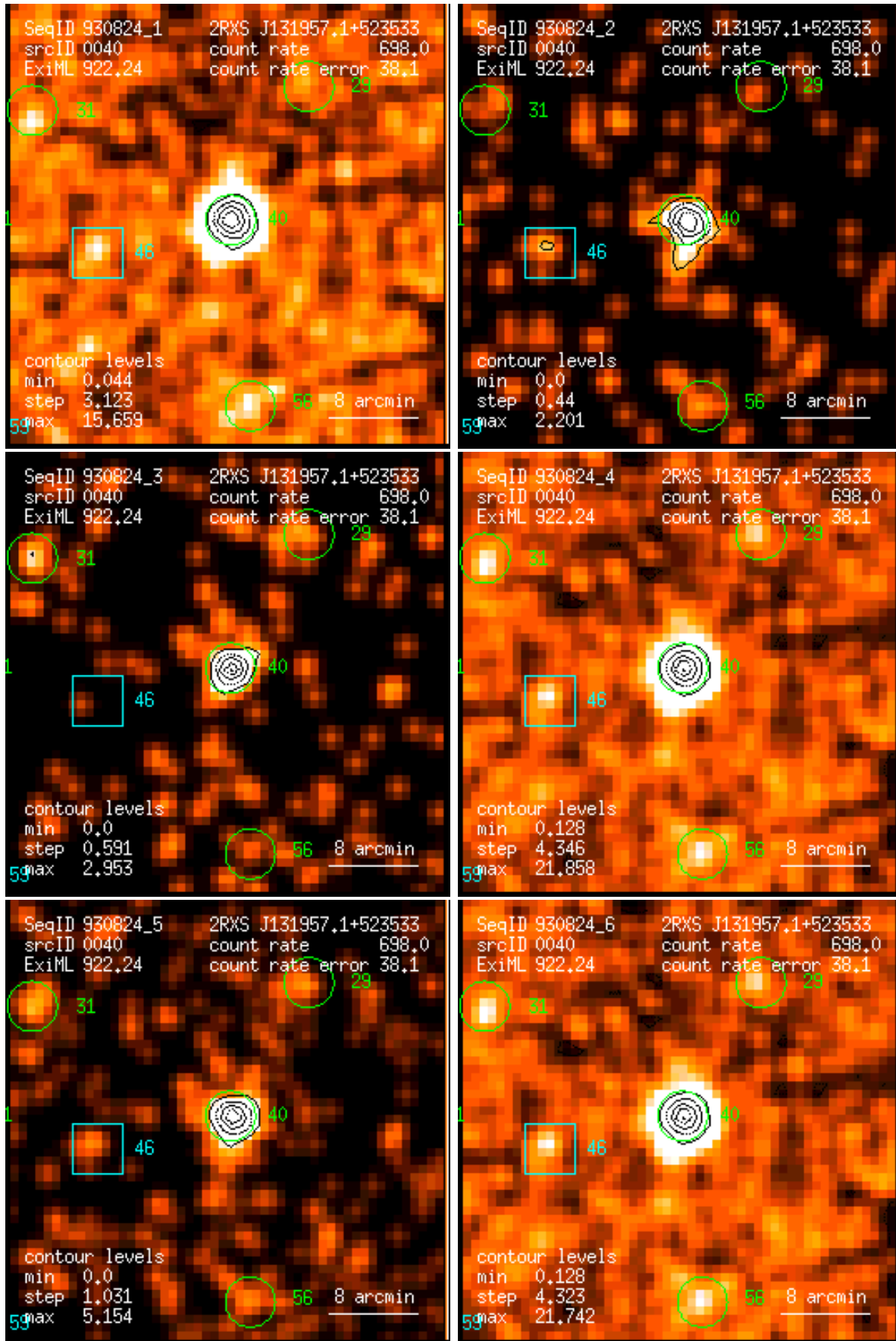
Figure 40: RASS 930824: detection 0040: band rate images, Gaussian filter: (1) PSPC channels 11 – 41, (2) 52 – 90, (3) 91 – 201, (4) 11 – 235, (5) 52 – 201, (6) 11 – 201. Broad band rates in counts/ks. Band rate contour levels in counts/ks/arcmin 2 .
