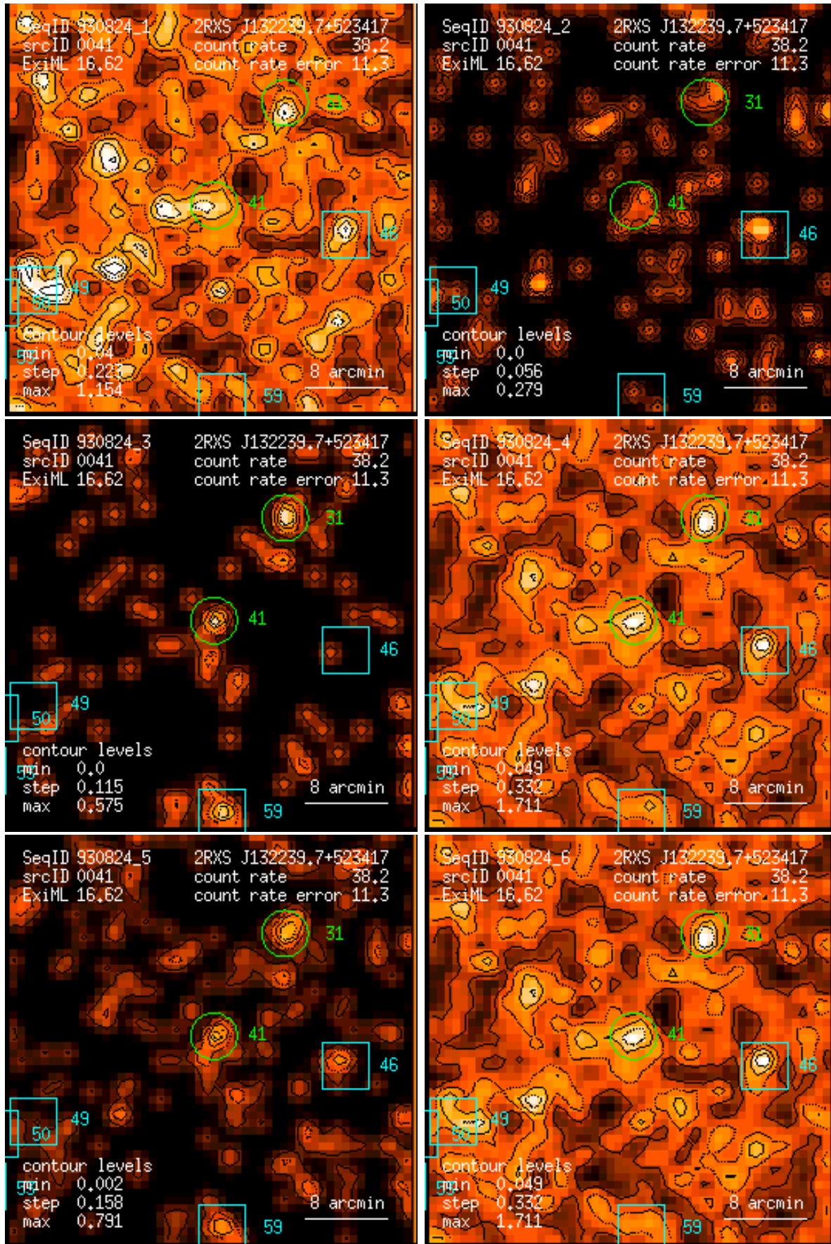
Figure 41: RASS 930824: detection 0041: band rate images, Gaussian filter: (1) PSPC channels 11 – 41, (2) 52 – 90, (3) 91 – 201, (4) 11 – 235, (5) 52 – 201, (6) 11 – 201. Broad band rates in counts/ks. Band rate contour levels in counts/ks/arcmin 2 .
