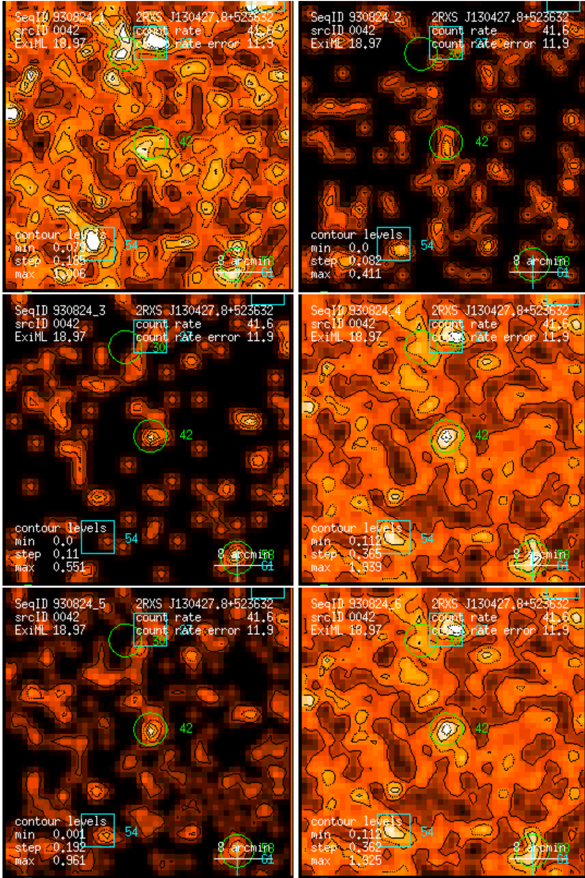
Figure 42: RASS 930824: detection 0042: band rate images, Gaussian filter: (1) PSPC channels 11 – 41, (2) 52 – 90, (3) 91 – 201, (4) 11 – 235, (5) 52 – 201, (6) 11 – 201. Broad band rates in counts/ks. Band rate contour levels in counts/ks/arcmin 2 .
