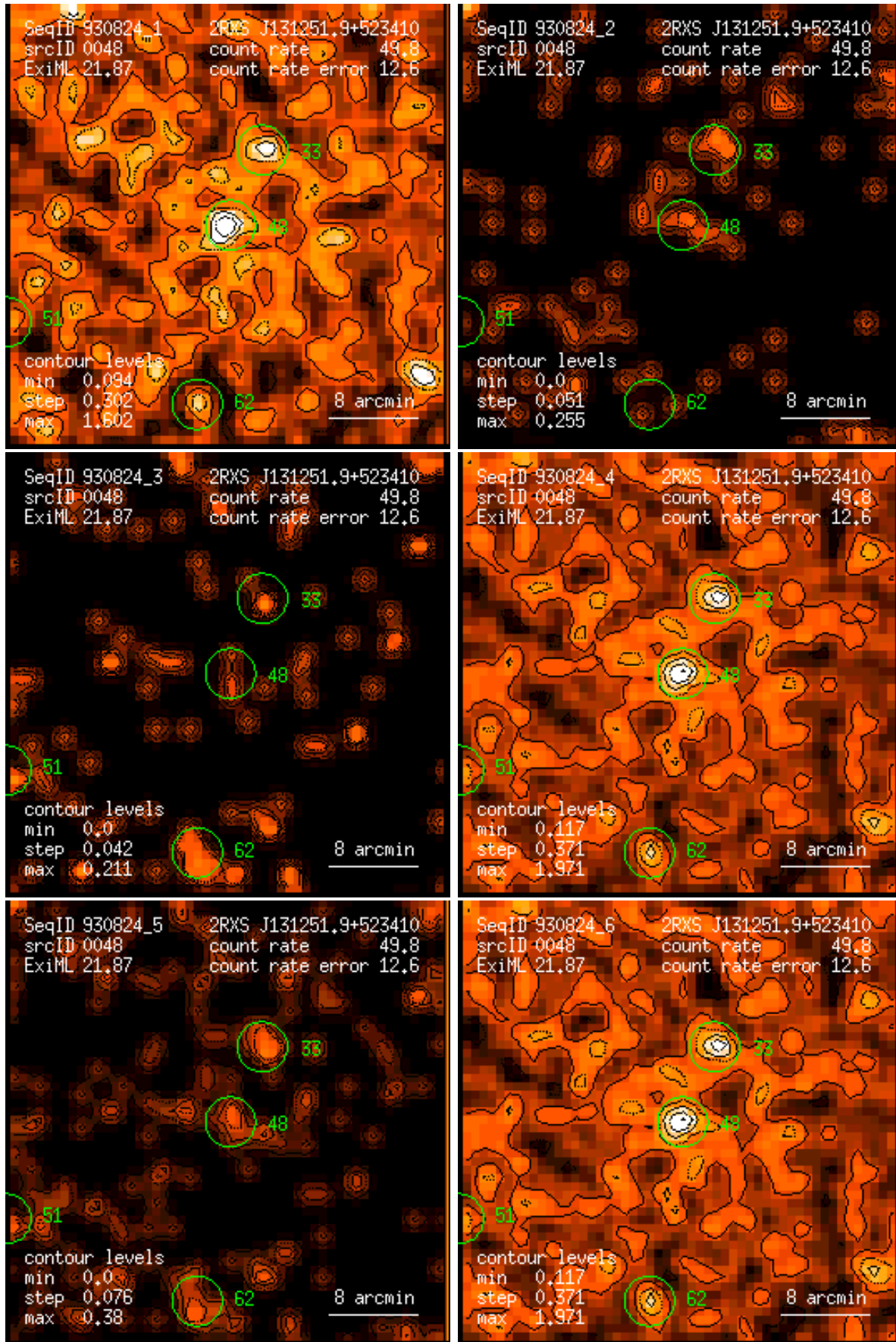
Figure 48: RASS 930824: detection 0048: band rate images, Gaussian filter: (1) PSPC channels 11 – 41, (2) 52 – 90, (3) 91 – 201, (4) 11 – 235, (5) 52 – 201, (6) 11 – 201. Broad band rates in counts/ks. Band rate contour levels in counts/ks/arcmin 2 .
