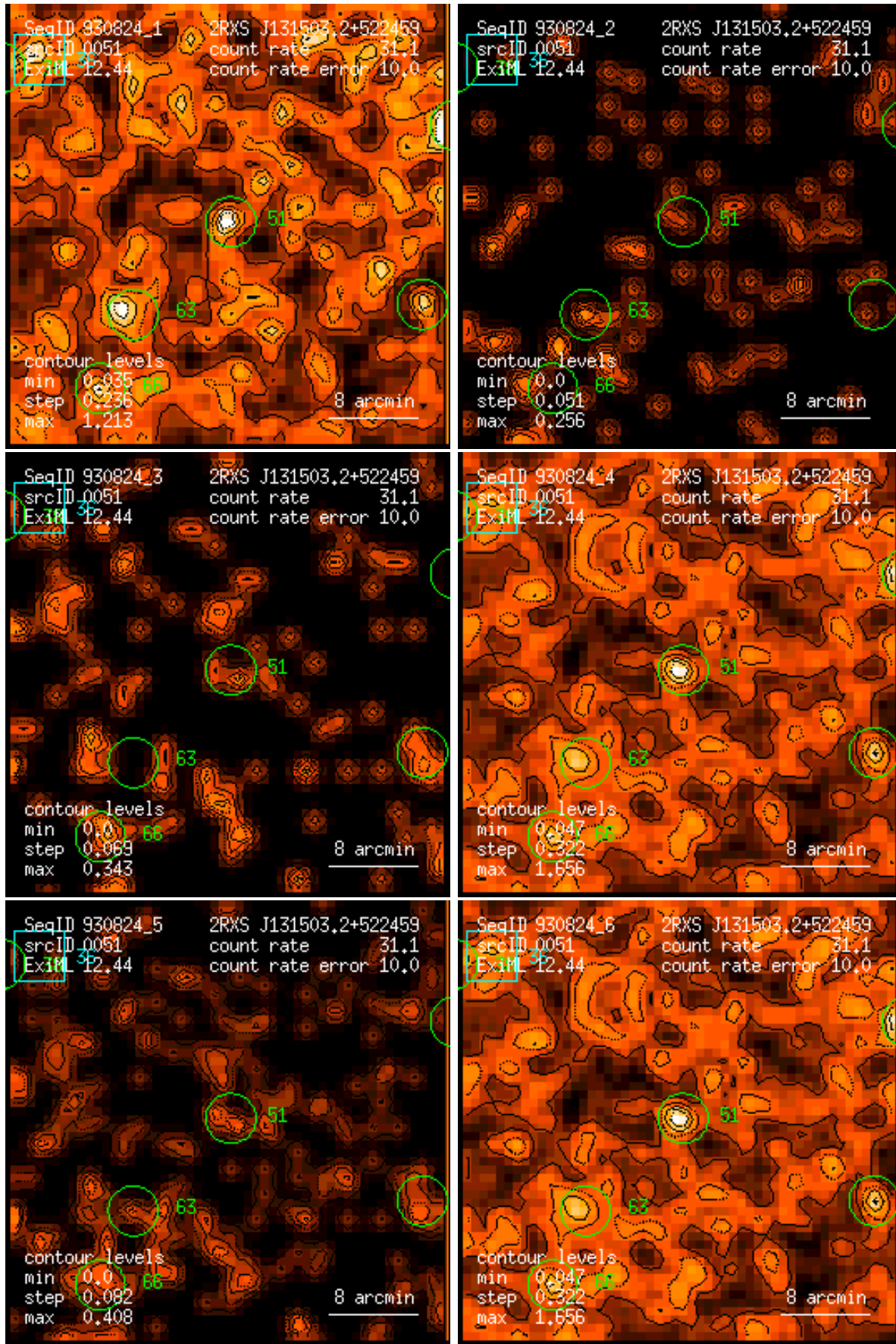
Figure 51: RASS 930824: detection 0051: band rate images, Gaussian filter: (1) PSPC channels 11 – 41, (2) 52 – 90, (3) 91 – 201, (4) 11 – 235, (5) 52 – 201, (6) 11 – 201. Broad band rates in counts/ks. Band rate contour levels in counts/ks/arcmin 2 .
