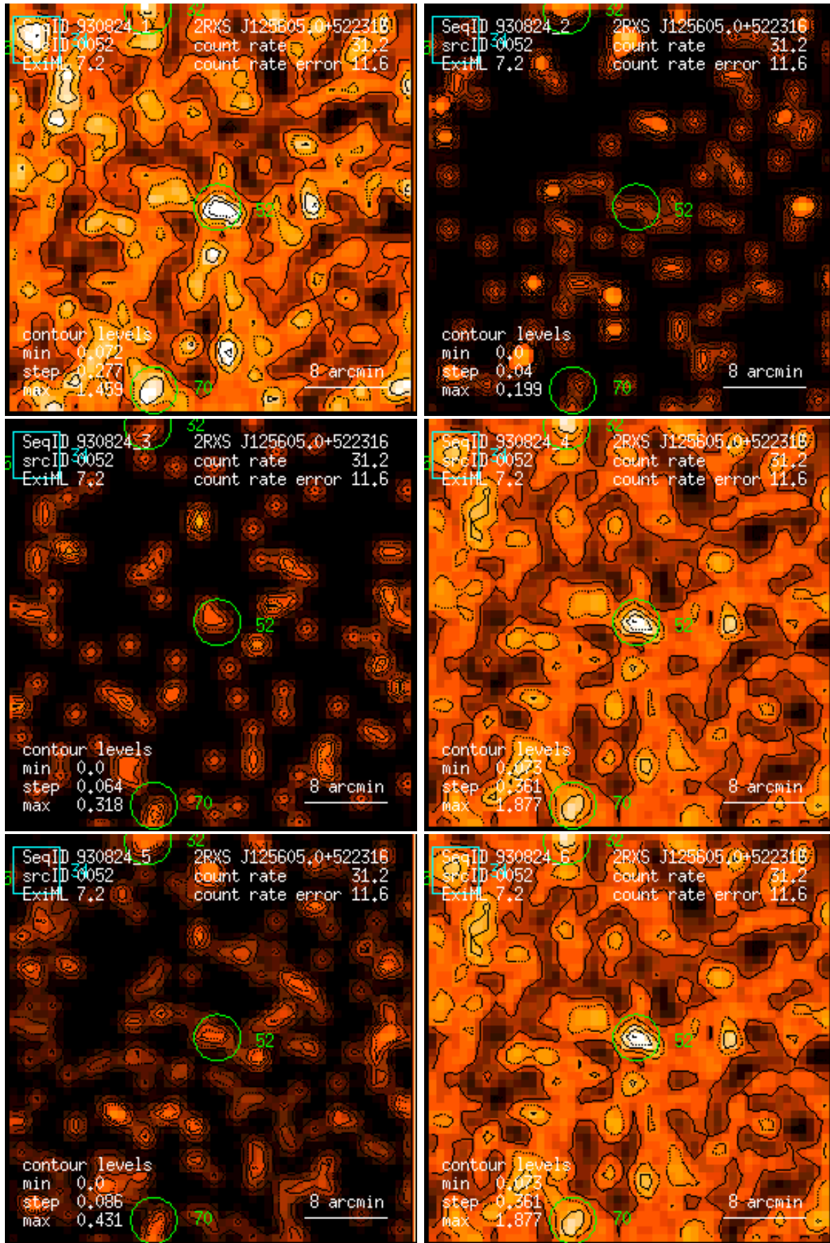
Figure 52: RASS 930824: detection 0052: band rate images, Gaussian filter: (1) PSPC channels 11 – 41, (2) 52 – 90, (3) 91 – 201, (4) 11 – 235, (5) 52 – 201, (6) 11 – 201. Broad band rates in counts/ks. Band rate contour levels in counts/ks/arcmin 2 .
