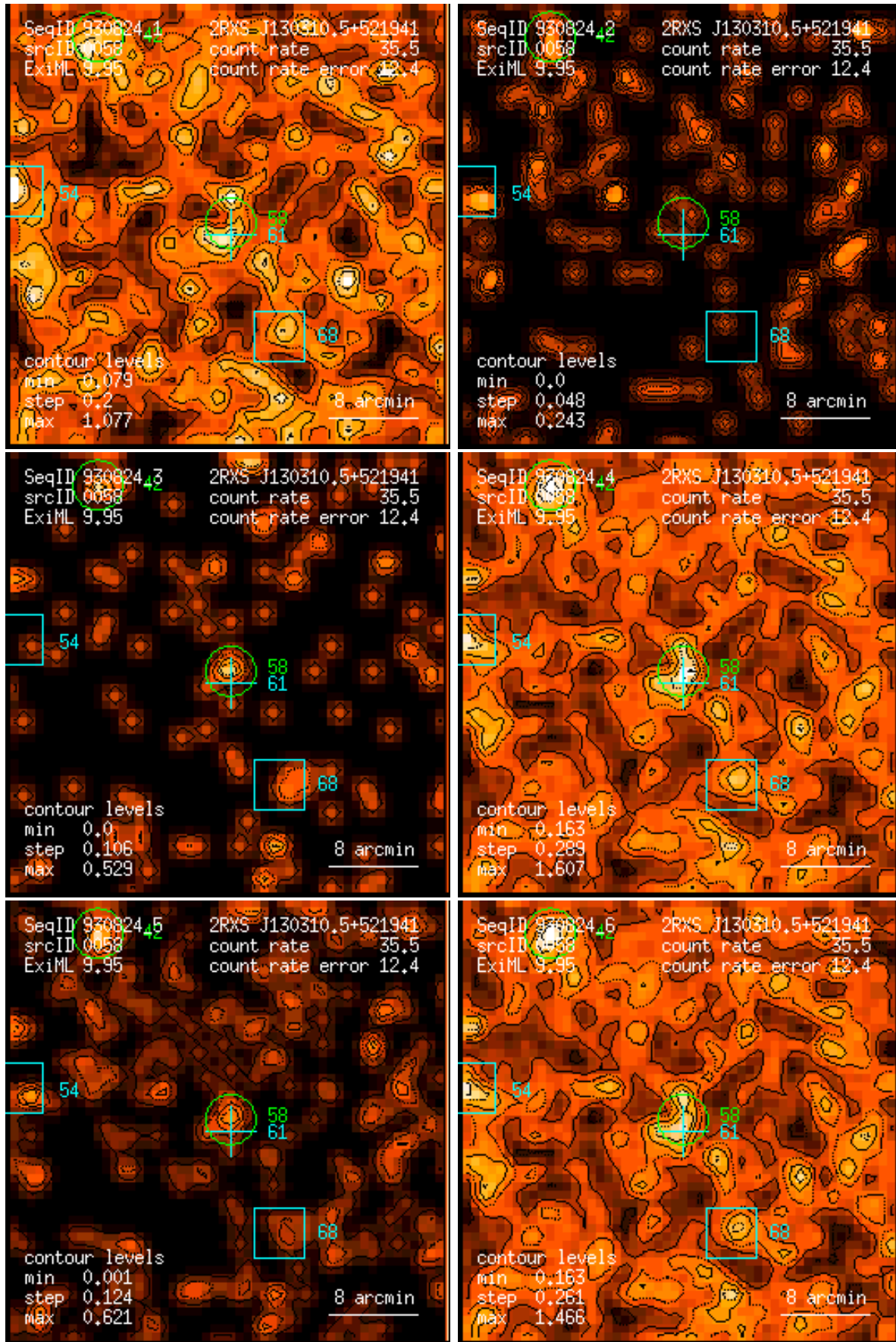
Figure 58: RASS 930824: detection 0058: band rate images, Gaussian filter: (1) PSPC channels 11 – 41, (2) 52 – 90, (3) 91 – 201, (4) 11 – 235, (5) 52 – 201, (6) 11 – 201. Broad band rates in counts/ks. Band rate contour levels in counts/ks/arcmin 2 .
