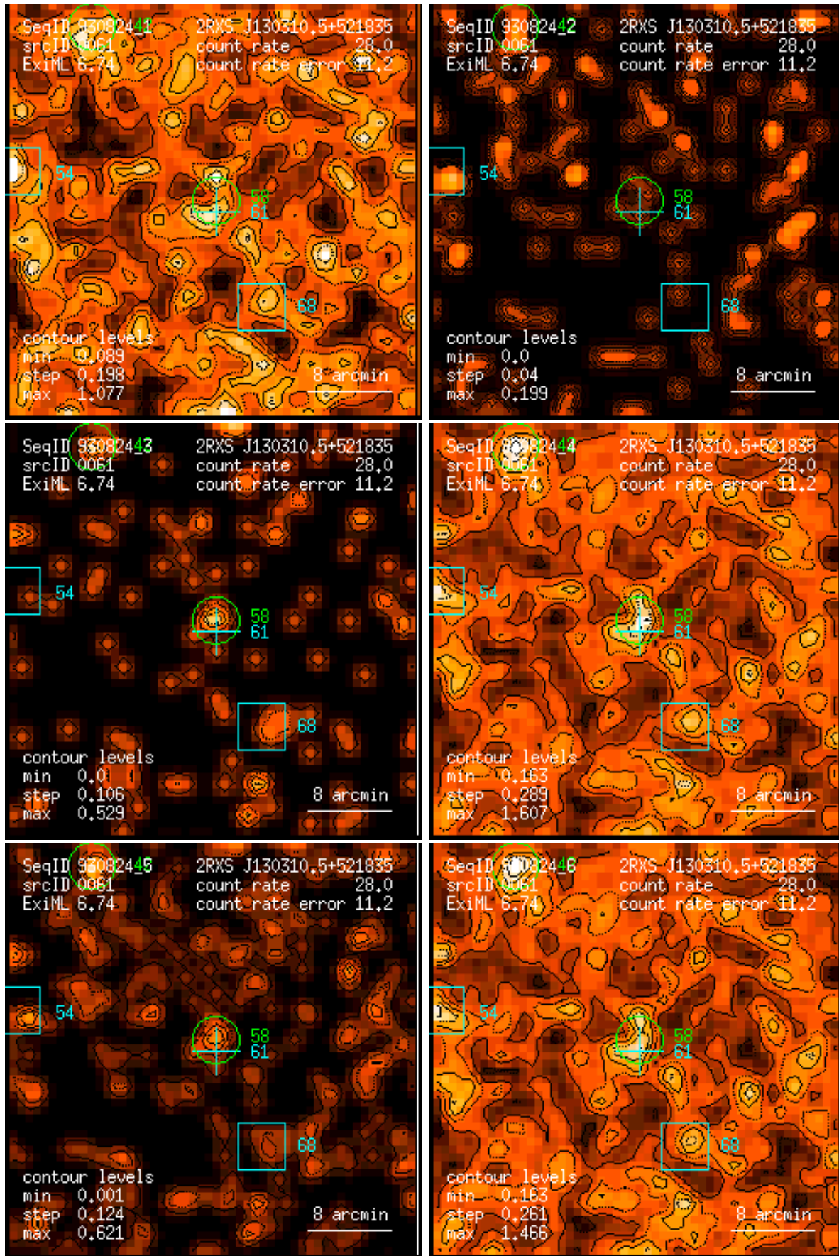
Figure 61: RASS 930824: detection 0061: band rate images, Gaussian filter: (1) PSPC channels 11 – 41, (2) 52 – 90, (3) 91 – 201, (4) 11 – 235, (5) 52 – 201, (6) 11 – 201. Broad band rates in counts/ks. Band rate contour levels in counts/ks/arcmin 2 .
