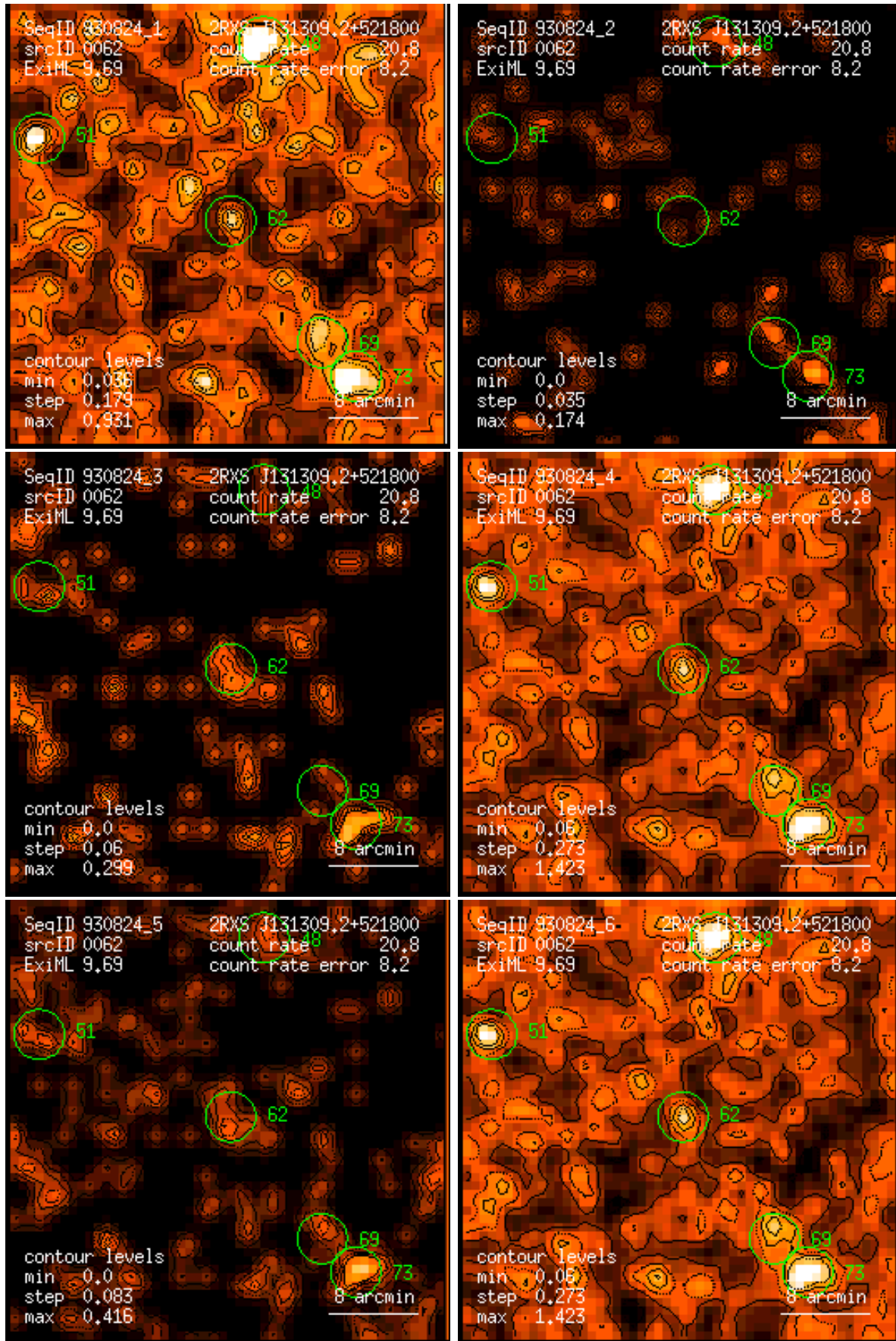
Figure 62: RASS 930824: detection 0062: band rate images, Gaussian filter: (1) PSPC channels 11 – 41, (2) 52 – 90, (3) 91 – 201, (4) 11 – 235, (5) 52 – 201, (6) 11 – 201. Broad band rates in counts/ks. Band rate contour levels in counts/ks/arcmin 2 .
