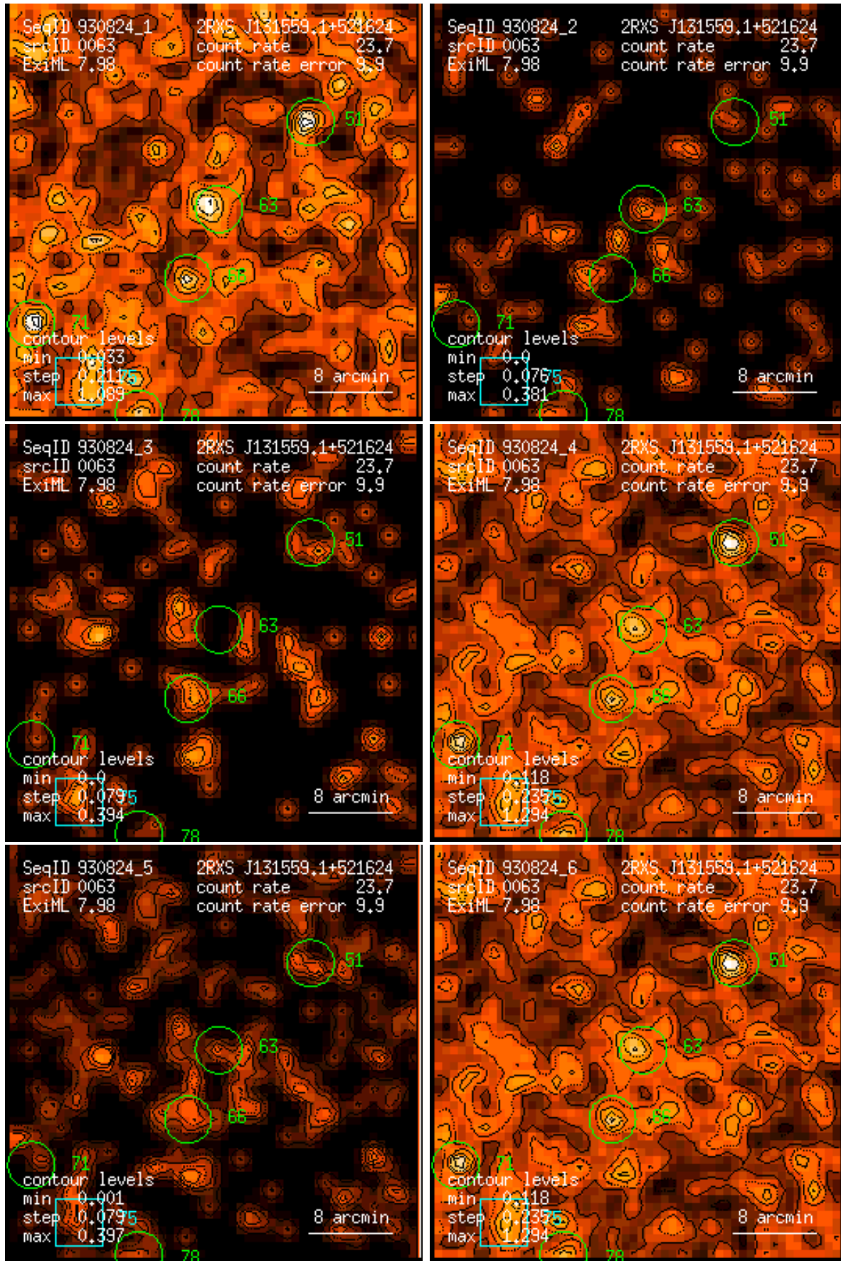
Figure 63: RASS 930824: detection 0063: band rate images, Gaussian filter: (1) PSPC channels 11 – 41, (2) 52 – 90, (3) 91 – 201, (4) 11 – 235, (5) 52 – 201, (6) 11 – 201. Broad band rates in counts/ks. Band rate contour levels in counts/ks/arcmin 2 .
