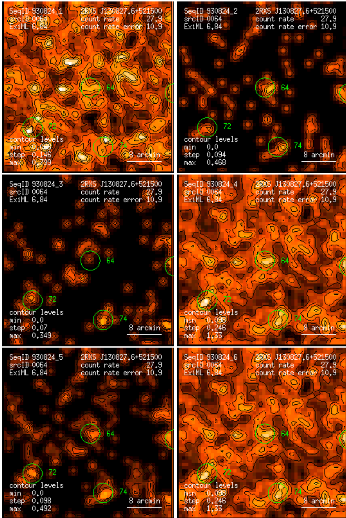
Figure 64: RASS 930824: detection 0064: band rate images, Gaussian filter: (1) PSPC channels 11 – 41, (2) 52 – 90, (3) 91 – 201, (4) 11 – 235, (5) 52 – 201, (6) 11 – 201. Broad band rates in counts/ks. Band rate contour levels in counts/ks/arcmin 2 .
