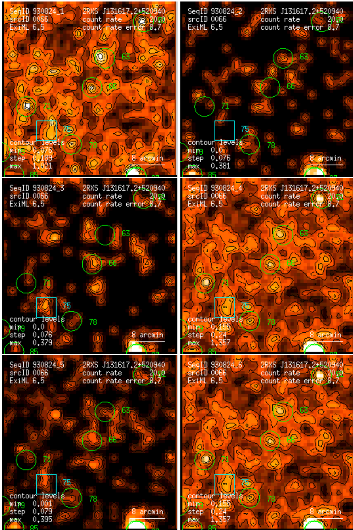
Figure 66: RASS 930824: detection 0066: band rate images, Gaussian filter: (1) PSPC channels 11 – 41, (2) 52 – 90, (3) 91 – 201, (4) 11 – 235, (5) 52 – 201, (6) 11 – 201. Broad band rates in counts/ks. Band rate contour levels in counts/ks/arcmin 2 .
