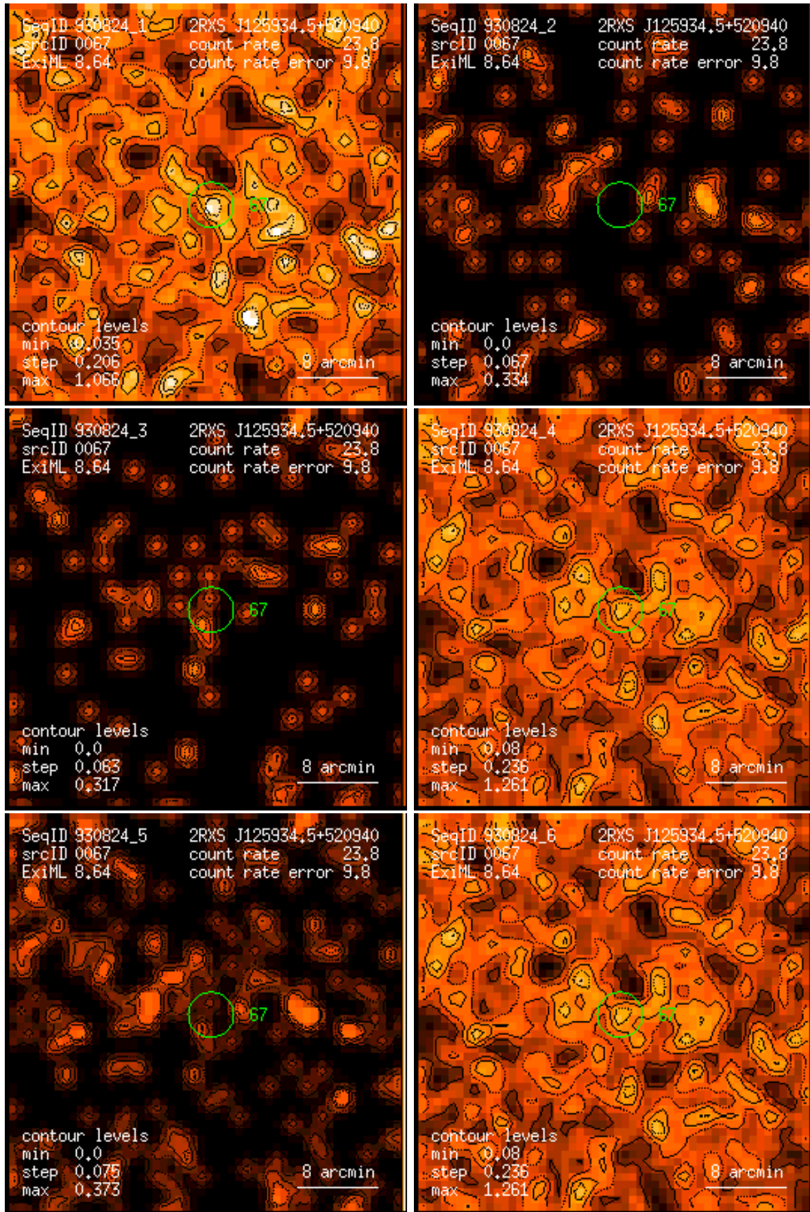
Figure 67: RASS 930824: detection 0067: band rate images, Gaussian filter: (1) PSPC channels 11 – 41, (2) 52 – 90, (3) 91 – 201, (4) 11 – 235, (5) 52 – 201, (6) 11 – 201. Broad band rates in counts/ks. Band rate contour levels in counts/ks/arcmin 2 .
