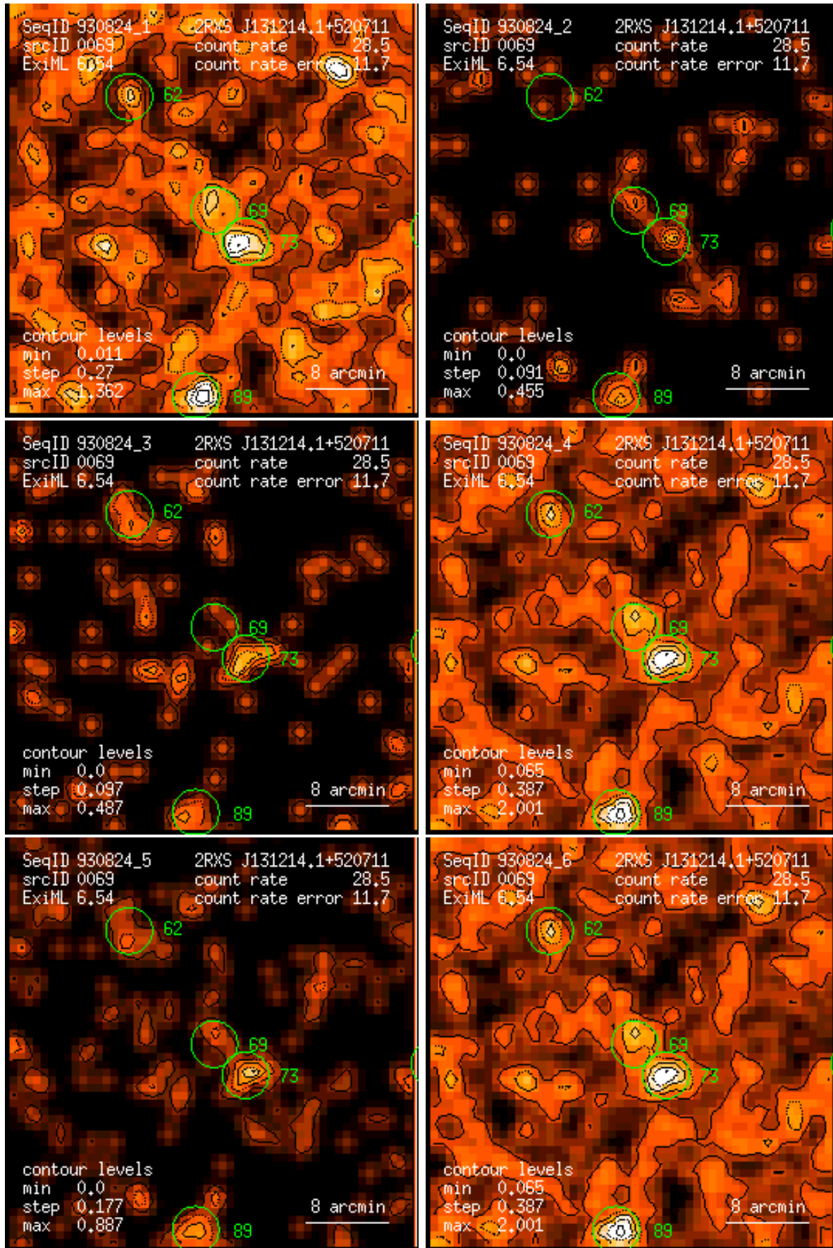
Figure 69: RASS 930824: detection 0069: band rate images, Gaussian filter: (1) PSPC channels 11 – 41, (2) 52 – 90, (3) 91 – 201, (4) 11 – 235, (5) 52 – 201, (6) 11 – 201. Broad band rates in counts/ks. Band rate contour levels in counts/ks/arcmin 2 .
