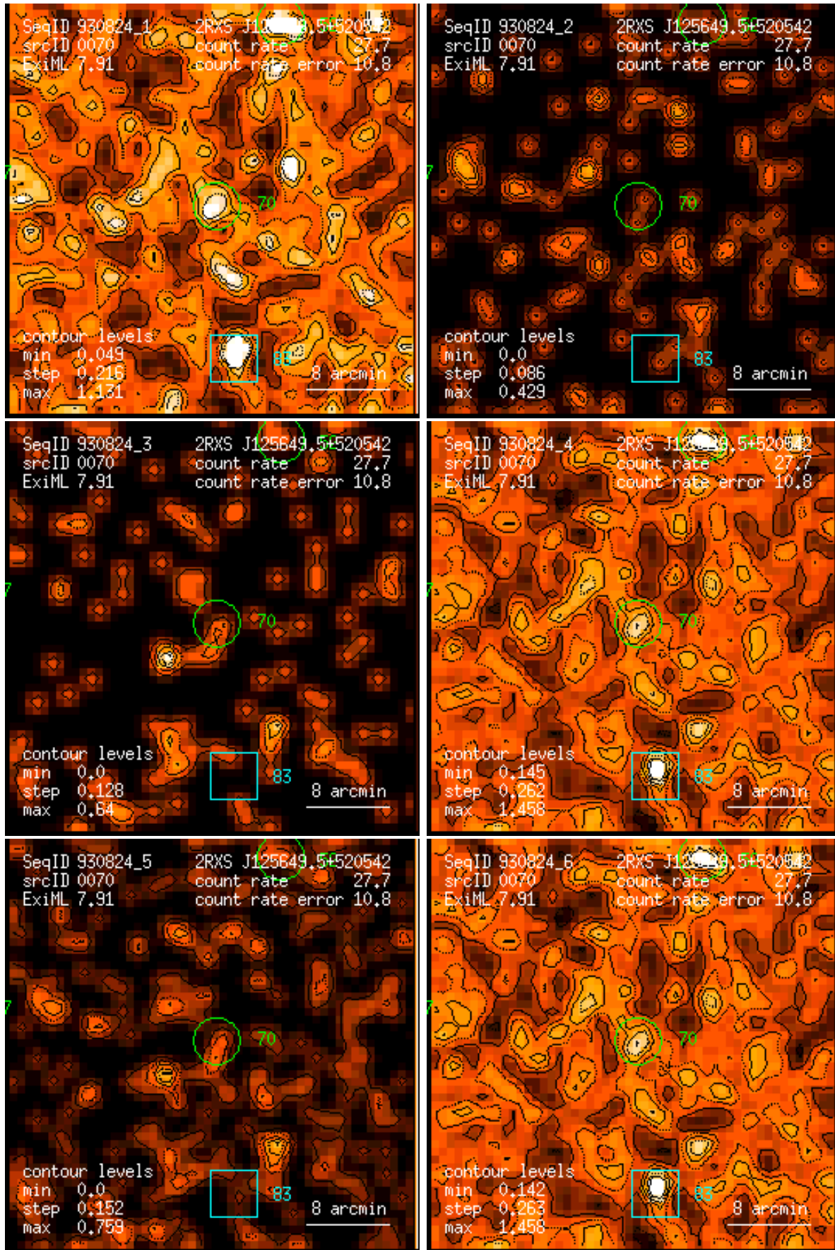
Figure 70: RASS 930824: detection 0070: band rate images, Gaussian filter: (1) PSPC channels 11 – 41, (2) 52 – 90, (3) 91 – 201, (4) 11 – 235, (5) 52 – 201, (6) 11 – 201. Broad band rates in counts/ks. Band rate contour levels in counts/ks/arcmin 2 .
