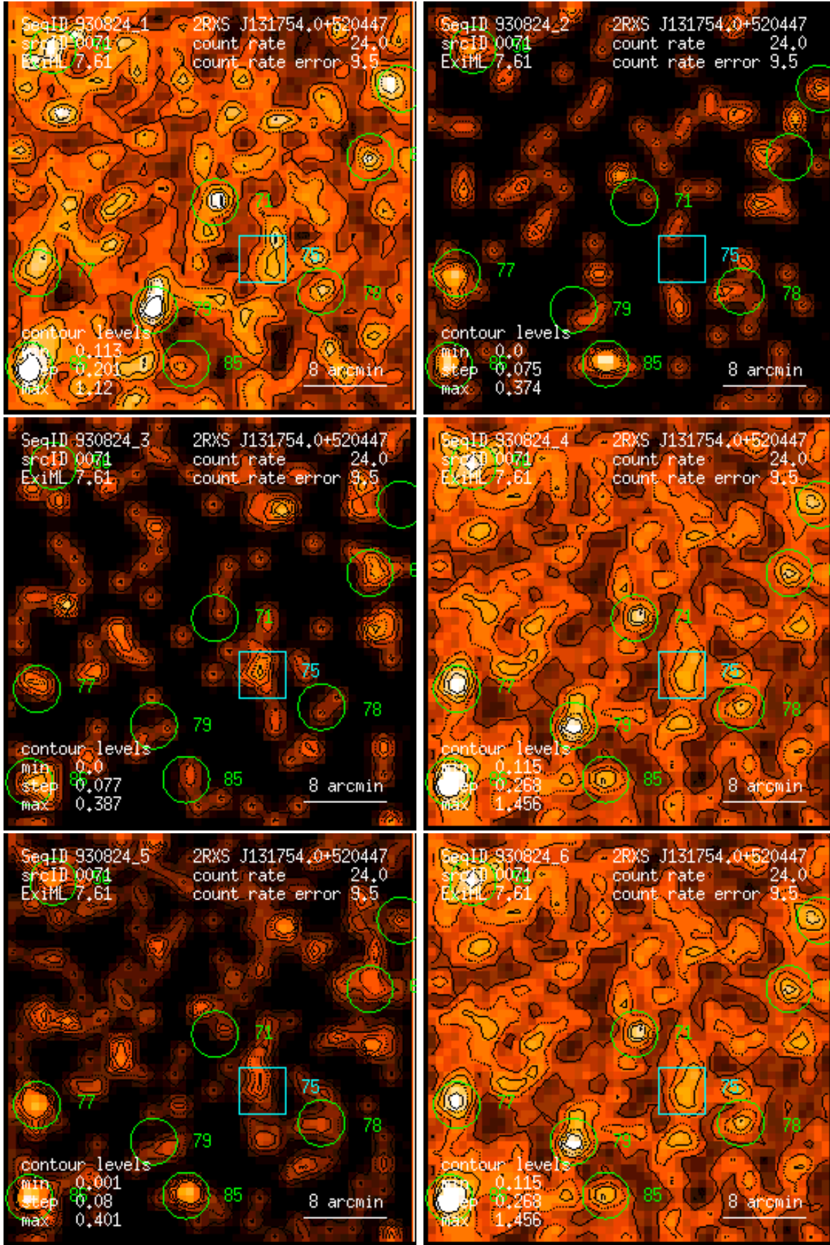
Figure 71: RASS 930824: detection 0071: band rate images, Gaussian filter: (1) PSPC channels 11 – 41, (2) 52 – 90, (3) 91 – 201, (4) 11 – 235, (5) 52 – 201, (6) 11 – 201. Broad band rates in counts/ks. Band rate contour levels in counts/ks/arcmin 2 .
