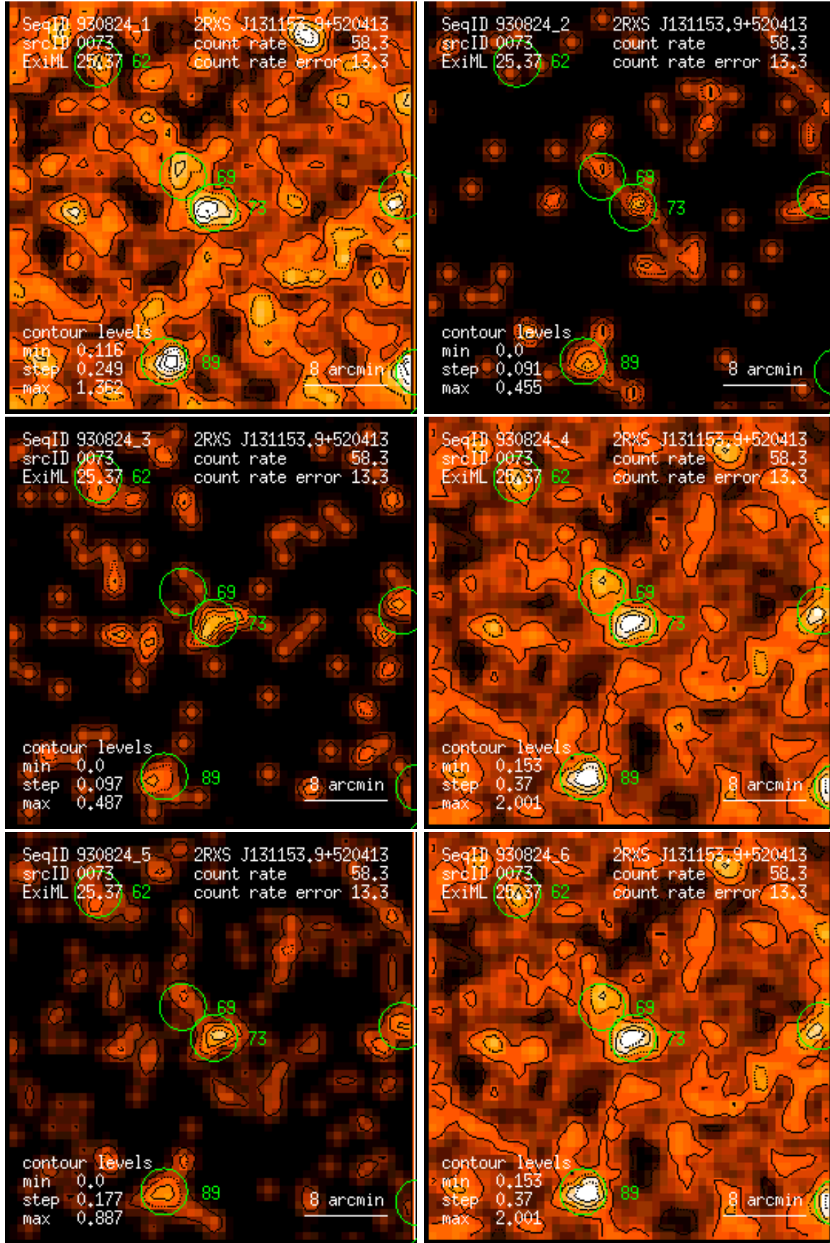
Figure 73: RASS 930824: detection 0073: band rate images, Gaussian filter: (1) PSPC channels 11 – 41, (2) 52 – 90, (3) 91 – 201, (4) 11 – 235, (5) 52 – 201, (6) 11 – 201. Broad band rates in counts/ks. Band rate contour levels in counts/ks/arcmin 2 .
