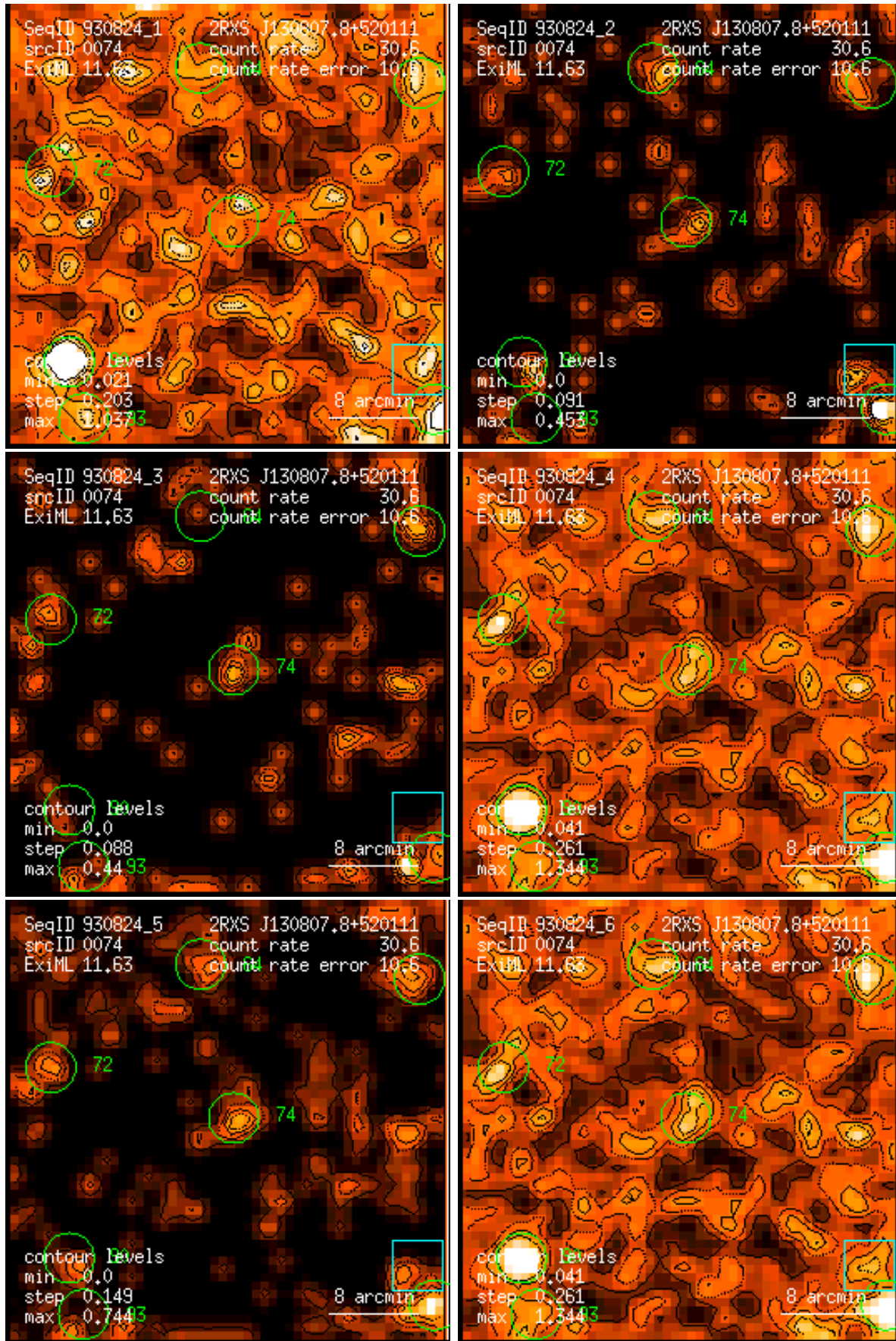
Figure 74: RASS 930824: detection 0074: band rate images, Gaussian filter: (1) PSPC channels 11 – 41, (2) 52 – 90, (3) 91 – 201, (4) 11 – 235, (5) 52 – 201, (6) 11 – 201. Broad band rates in counts/ks. Band rate contour levels in counts/ks/arcmin 2 .
