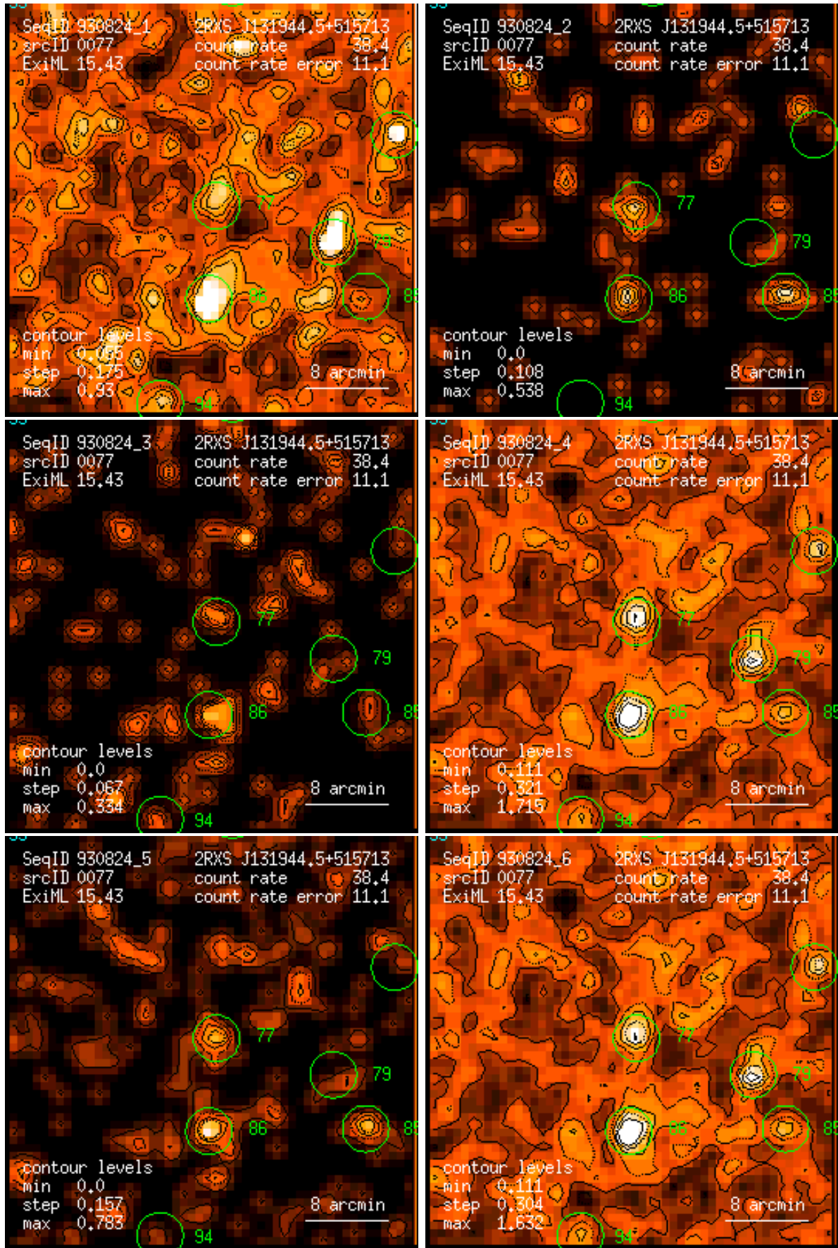
Figure 77: RASS 930824: detection 0077: band rate images, Gaussian filter: (1) PSPC channels 11 – 41, (2) 52 – 90, (3) 91 – 201, (4) 11 – 235, (5) 52 – 201, (6) 11 – 201. Broad band rates in counts/ks. Band rate contour levels in counts/ks/arcmin 2 .
