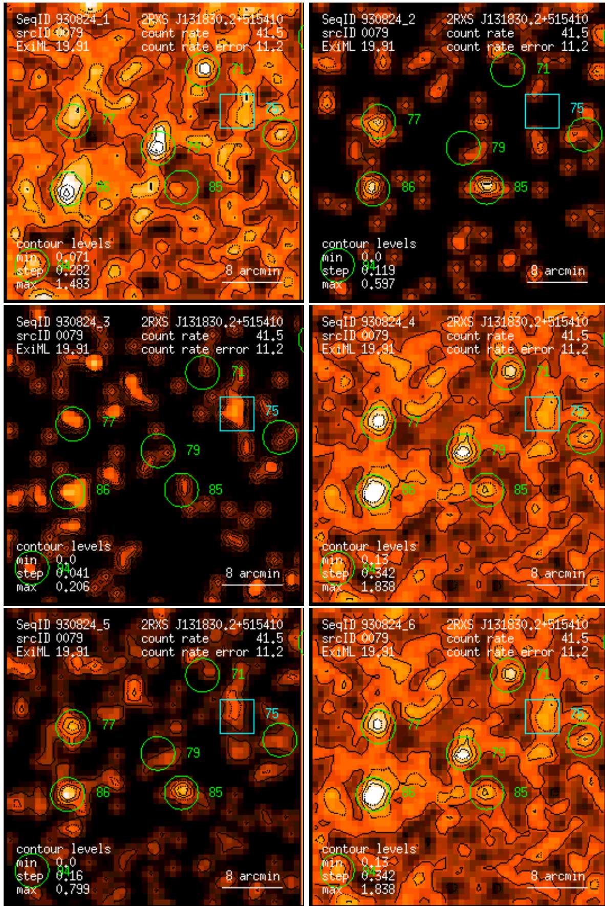
Figure 79: RASS 930824: detection 0079: band rate images, Gaussian filter: (1) PSPC channels 11 – 41, (2) 52 – 90, (3) 91 – 201, (4) 11 – 235, (5) 52 – 201, (6) 11 – 201. Broad band rates in counts/ks. Band rate contour levels in counts/ks/arcmin 2 .
