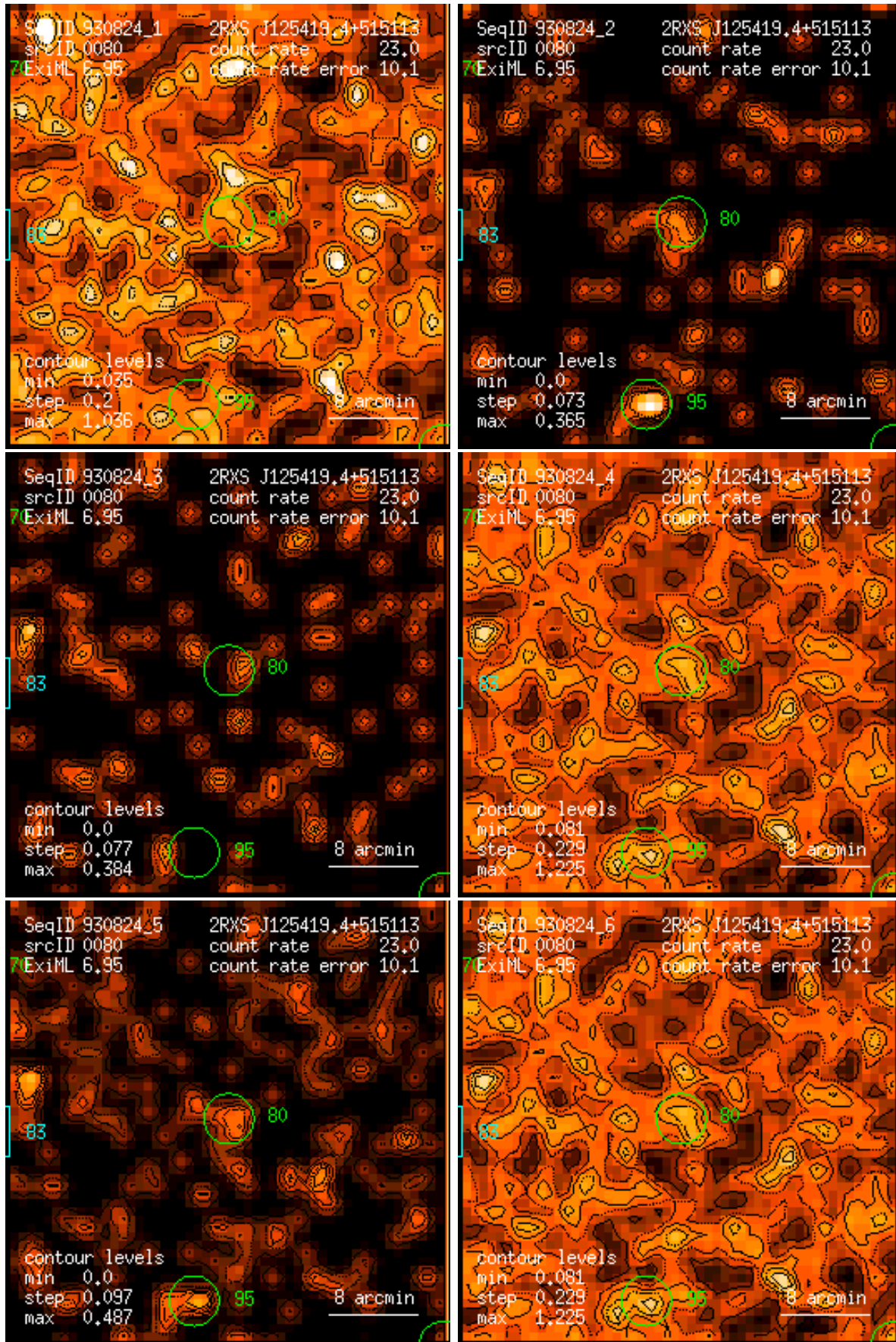
Figure 80: RASS 930824: detection 0080: band rate images, Gaussian filter: (1) PSPC channels 11 – 41, (2) 52 – 90, (3) 91 – 201, (4) 11 – 235, (5) 52 – 201, (6) 11 – 201. Broad band rates in counts/ks. Band rate contour levels in counts/ks/arcmin 2 .
