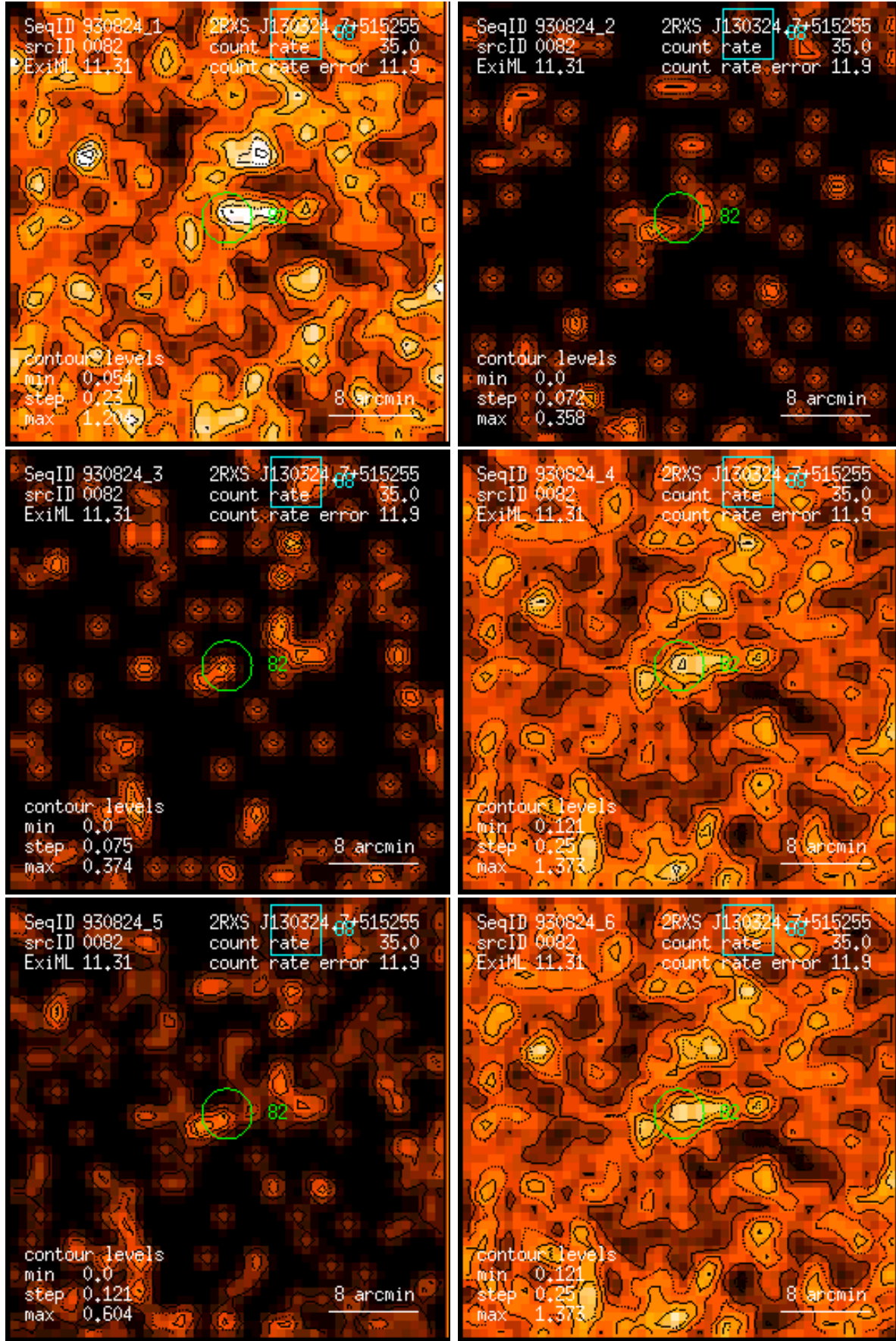
Figure 82: RASS 930824: detection 0082: band rate images, Gaussian filter: (1) PSPC channels 11 – 41, (2) 52 – 90, (3) 91 – 201, (4) 11 – 235, (5) 52 – 201, (6) 11 – 201. Broad band rates in counts/ks. Band rate contour levels in counts/ks/arcmin 2 .
