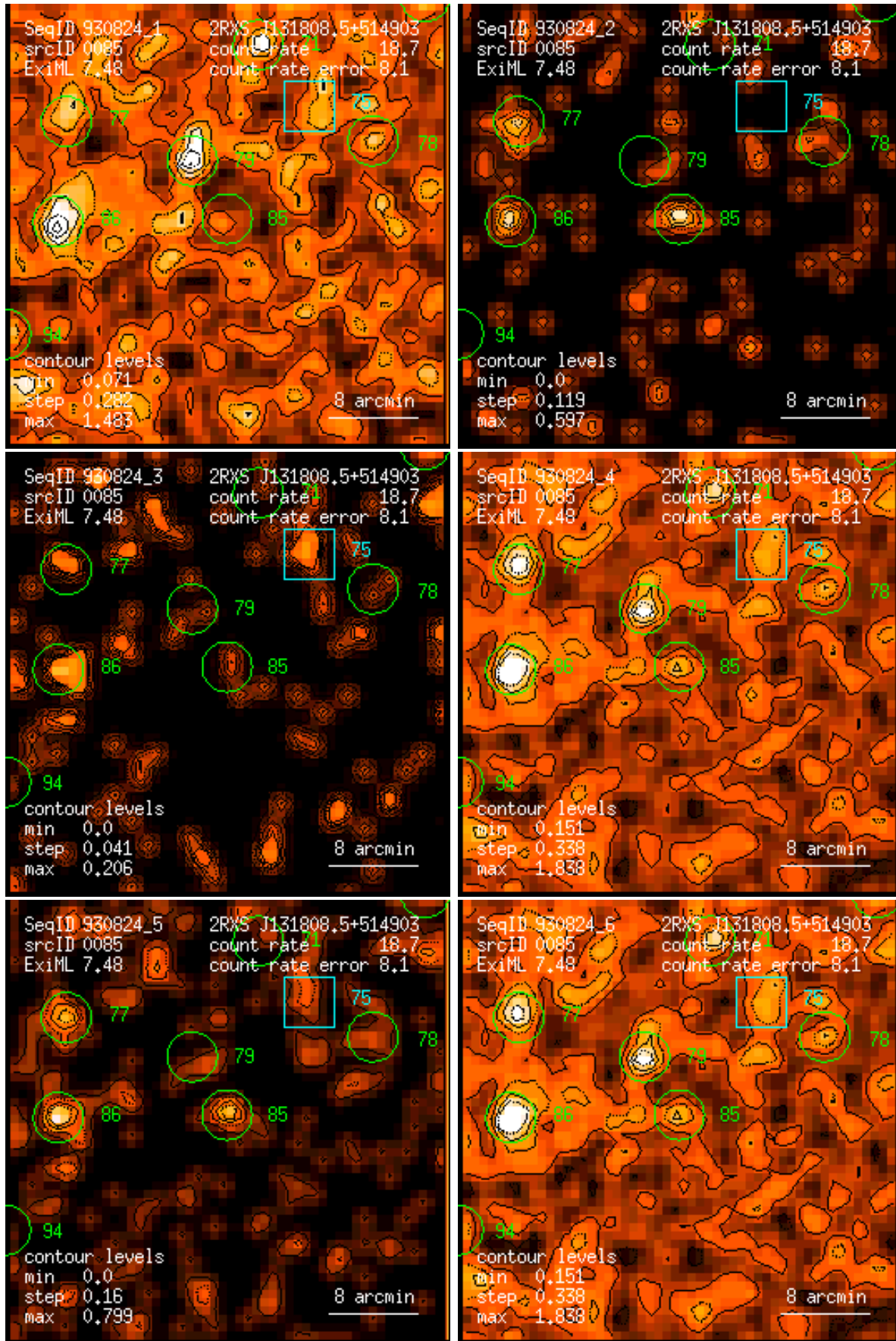
Figure 85: RASS 930824: detection 0085: band rate images, Gaussian filter: (1) PSPC channels 11 – 41, (2) 52 – 90, (3) 91 – 201, (4) 11 – 235, (5) 52 – 201, (6) 11 – 201. Broad band rates in counts/ks. Band rate contour levels in counts/ks/arcmin 2 .
