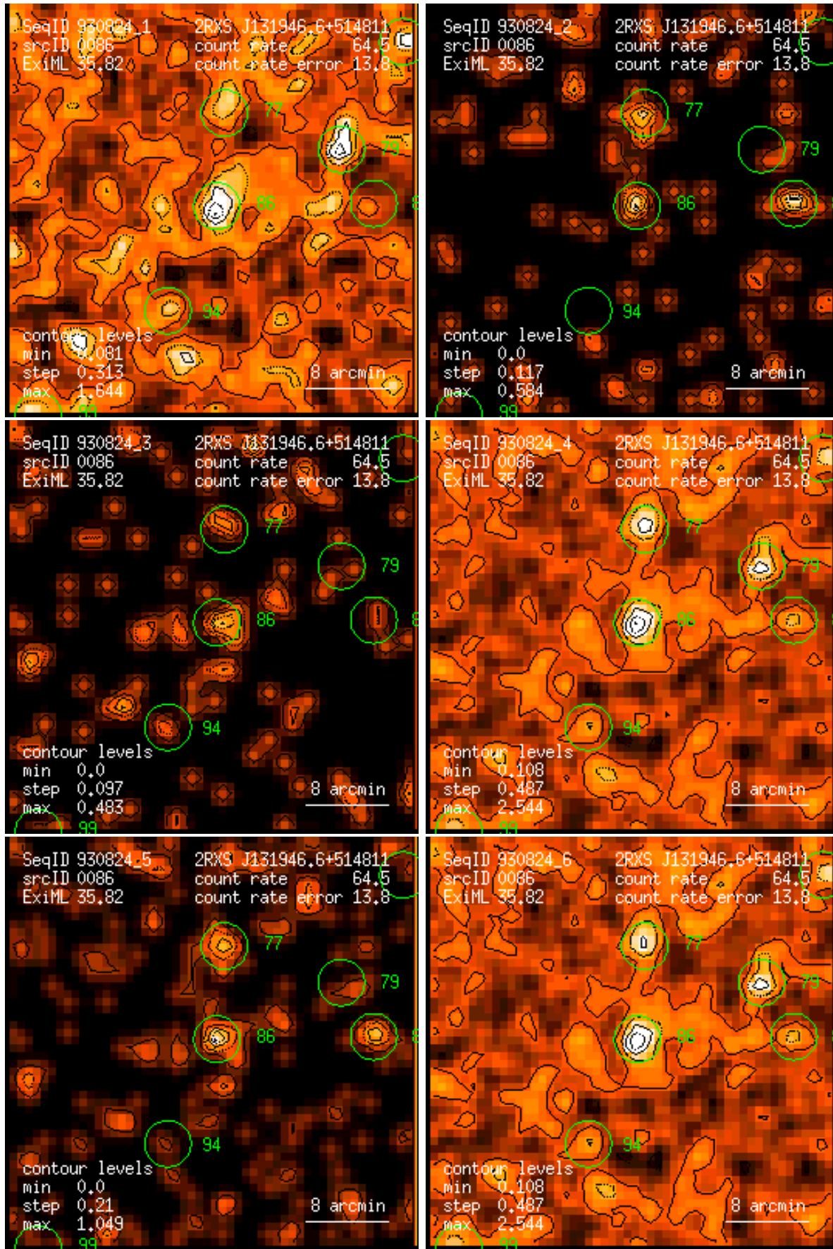
Figure 86: RASS 930824: detection 0086: band rate images, Gaussian filter: (1) PSPC channels 11 – 41, (2) 52 – 90, (3) 91 – 201, (4) 11 – 235, (5) 52 – 201, (6) 11 – 201. Broad band rates in counts/ks. Band rate contour levels in counts/ks/arcmin 2 .
