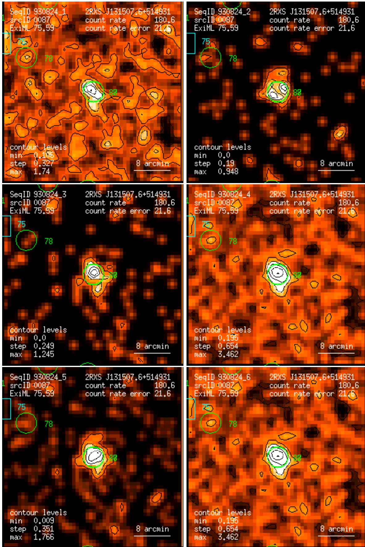
Figure 87: RASS 930824: detection 0087: band rate images, Gaussian filter: (1) PSPC channels 11 – 41, (2) 52 – 90, (3) 91 – 201, (4) 11 – 235, (5) 52 – 201, (6) 11 – 201. Broad band rates in counts/ks. Band rate contour levels in counts/ks/arcmin 2 .
