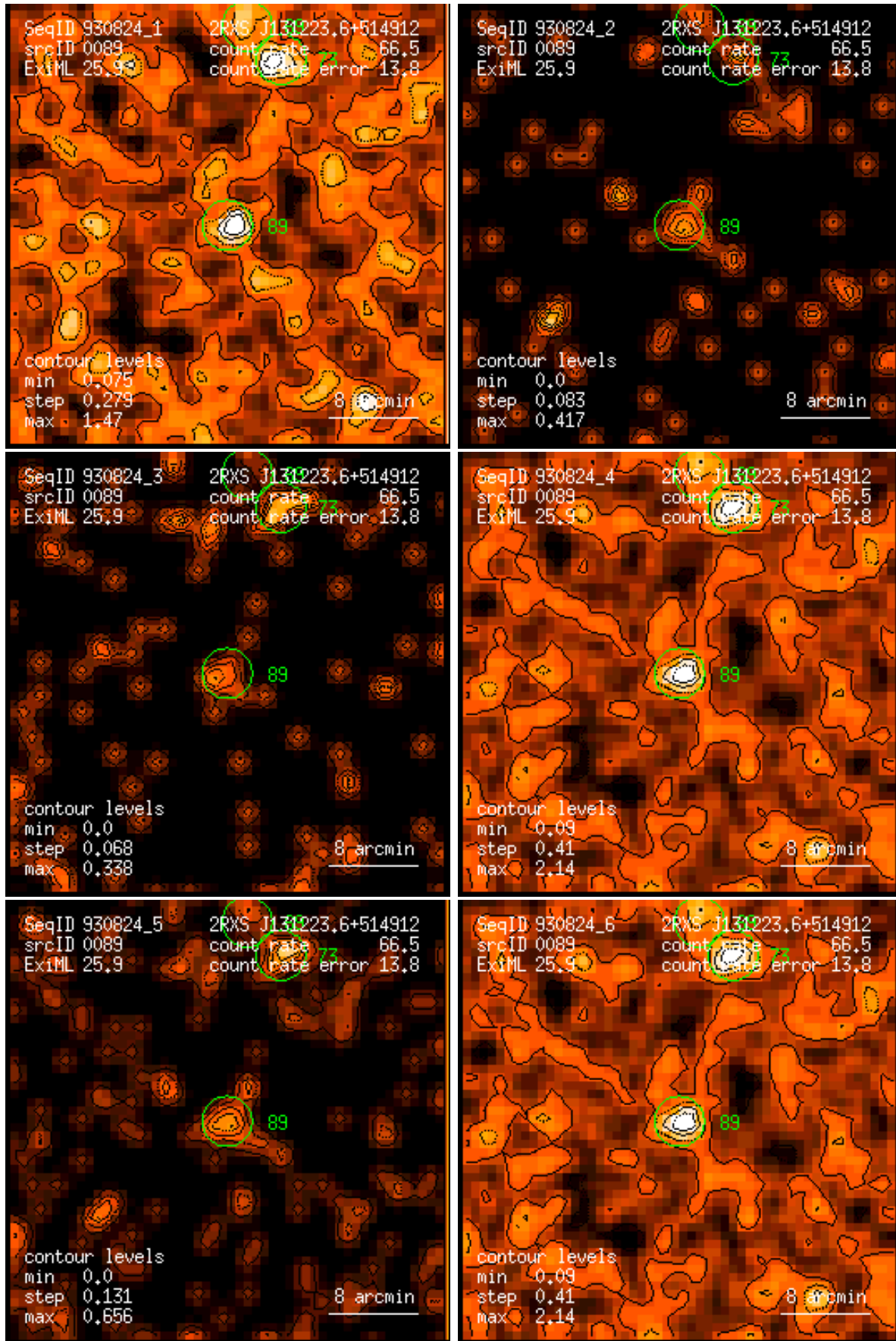
Figure 89: RASS 930824: detection 0089: band rate images, Gaussian filter: (1) PSPC channels 11 – 41, (2) 52 – 90, (3) 91 – 201, (4) 11 – 235, (5) 52 – 201, (6) 11 – 201. Broad band rates in counts/ks. Band rate contour levels in counts/ks/arcmin 2 .
