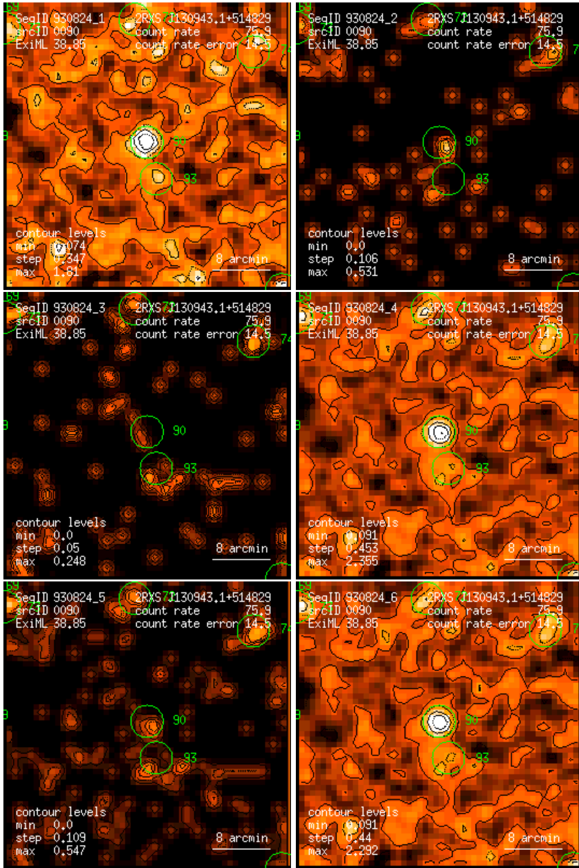
Figure 90: RASS 930824: detection 0090: band rate images, Gaussian filter: (1) PSPC channels 11 – 41, (2) 52 – 90, (3) 91 – 201, (4) 11 – 235, (5) 52 – 201, (6) 11 – 201. Broad band rates in counts/ks. Band rate contour levels in counts/ks/arcmin 2 .
