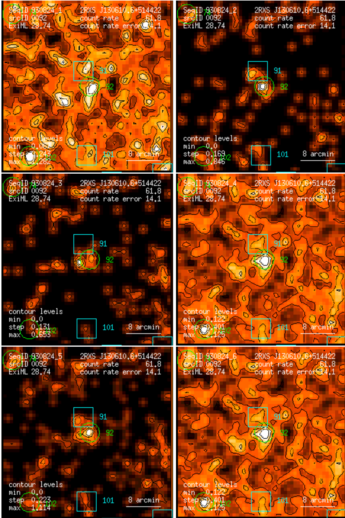
Figure 92: RASS 930824: detection 0092: band rate images, Gaussian filter: (1) PSPC channels 11 – 41, (2) 52 – 90, (3) 91 – 201, (4) 11 – 235, (5) 52 – 201, (6) 11 – 201. Broad band rates in counts/ks. Band rate contour levels in counts/ks/arcmin 2 .
