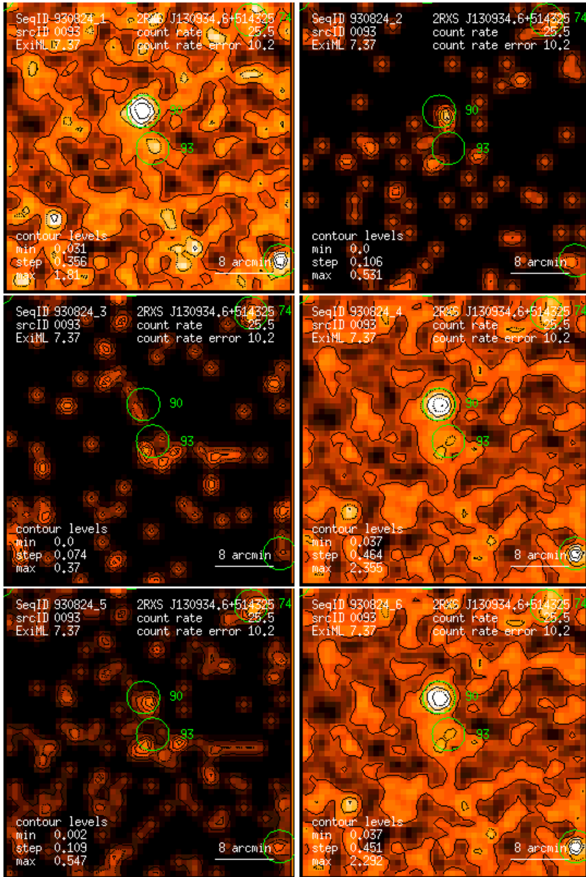
Figure 93: RASS 930824: detection 0093: band rate images, Gaussian filter: (1) PSPC channels 11 – 41, (2) 52 – 90, (3) 91 – 201, (4) 11 – 235, (5) 52 – 201, (6) 11 – 201. Broad band rates in counts/ks. Band rate contour levels in counts/ks/arcmin 2 .
