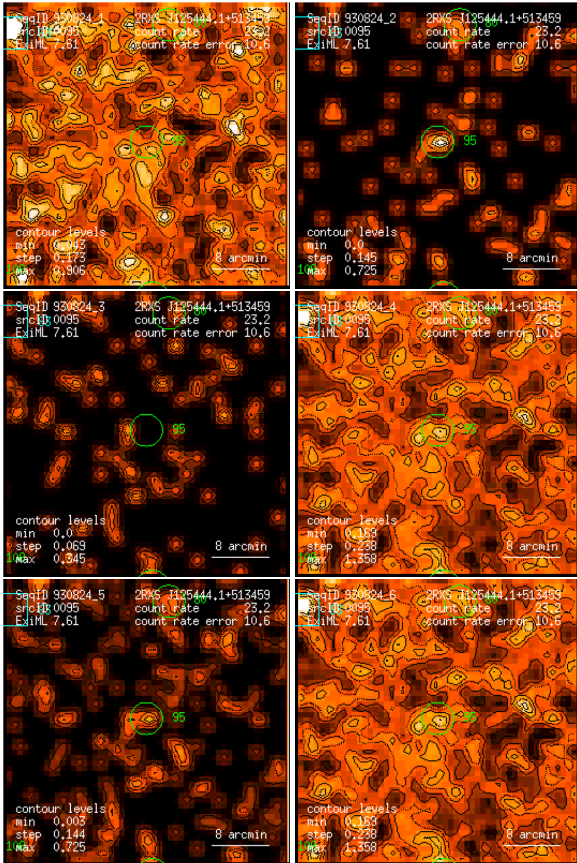
Figure 95: RASS 930824: detection 0095: band rate images, Gaussian filter: (1) PSPC channels 11 – 41, (2) 52 – 90, (3) 91 – 201, (4) 11 – 235, (5) 52 – 201, (6) 11 – 201. Broad band rates in counts/ks. Band rate contour levels in counts/ks/arcmin 2 .
