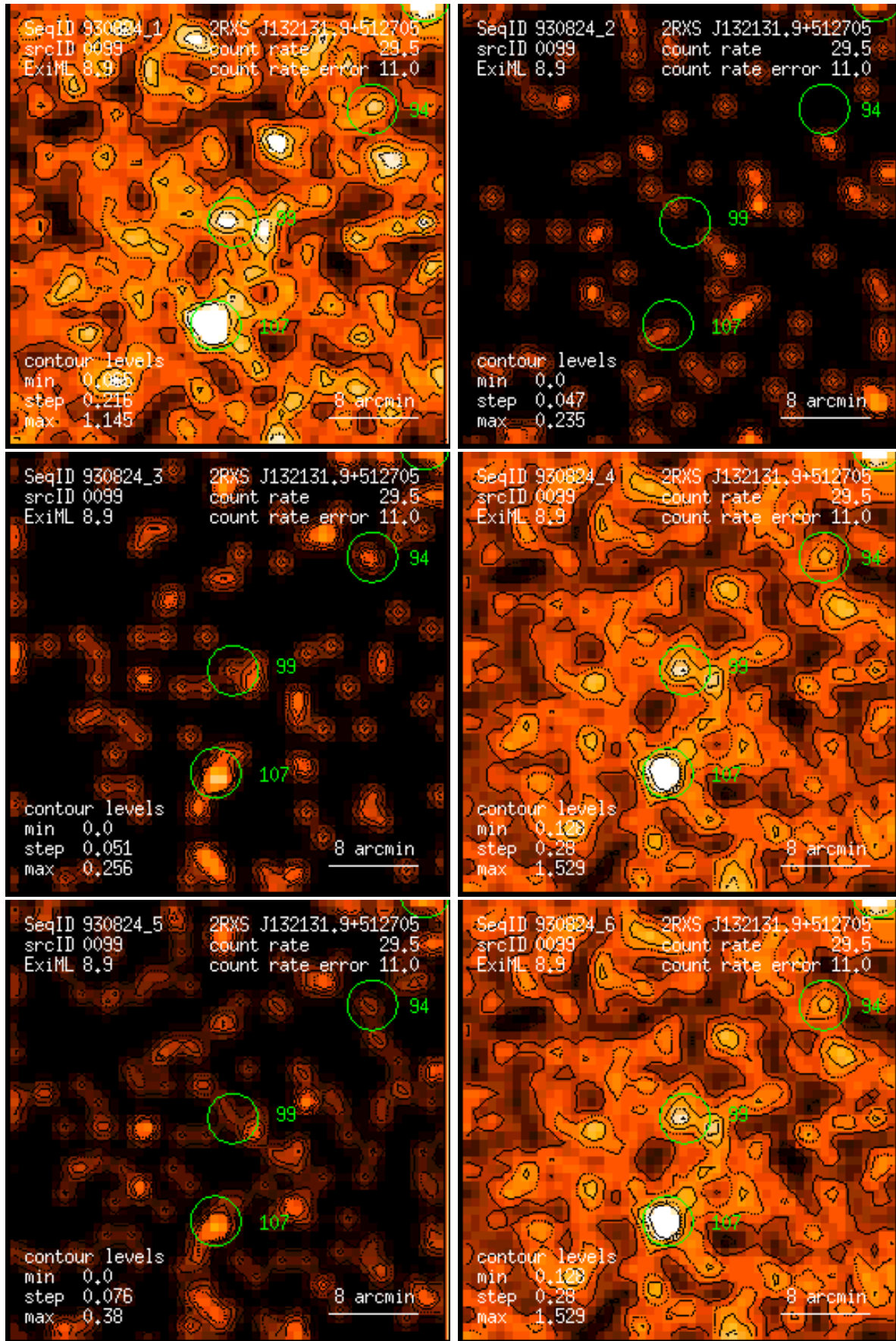
Figure 99: RASS 930824: detection 0099: band rate images, Gaussian filter: (1) PSPC channels 11 – 41, (2) 52 – 90, (3) 91 – 201, (4) 11 – 235, (5) 52 – 201, (6) 11 – 201. Broad band rates in counts/ks. Band rate contour levels in counts/ks/arcmin 2 .
