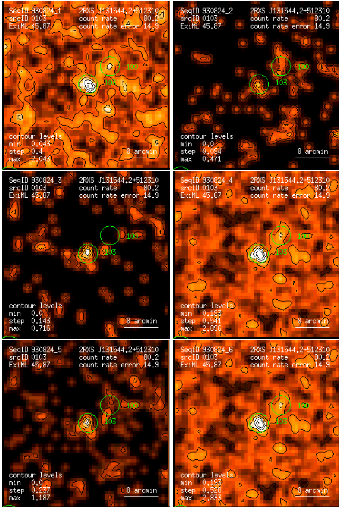
Figure 103: RASS 930824: detection 0103: band rate images, Gaussian filter: (1) PSPC channels 11 – 41, (2) 52 – 90, (3) 91 – 201, (4) 11 – 235, (5) 52 – 201, (6) 11 – 201. Broad band rates in counts/ks. Band rate contour levels in counts/ks/arcmin 2 .
