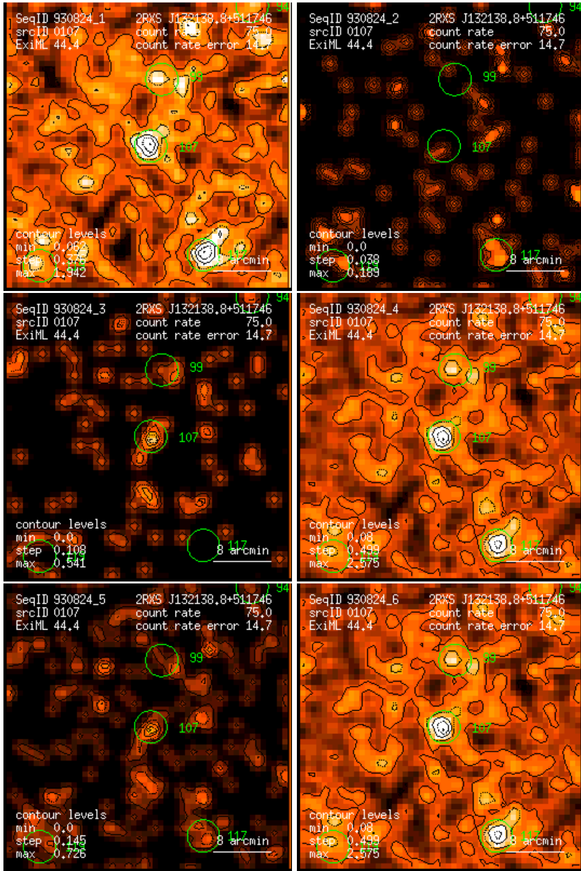
Figure 107: RASS 930824: detection 0107: band rate images, Gaussian filter: (1) PSPC channels 11 – 41, (2) 52 – 90, (3) 91 – 201, (4) 11 – 235, (5) 52 – 201, (6) 11 – 201. Broad band rates in counts/ks. Band rate contour levels in counts/ks/arcmin 2 .
