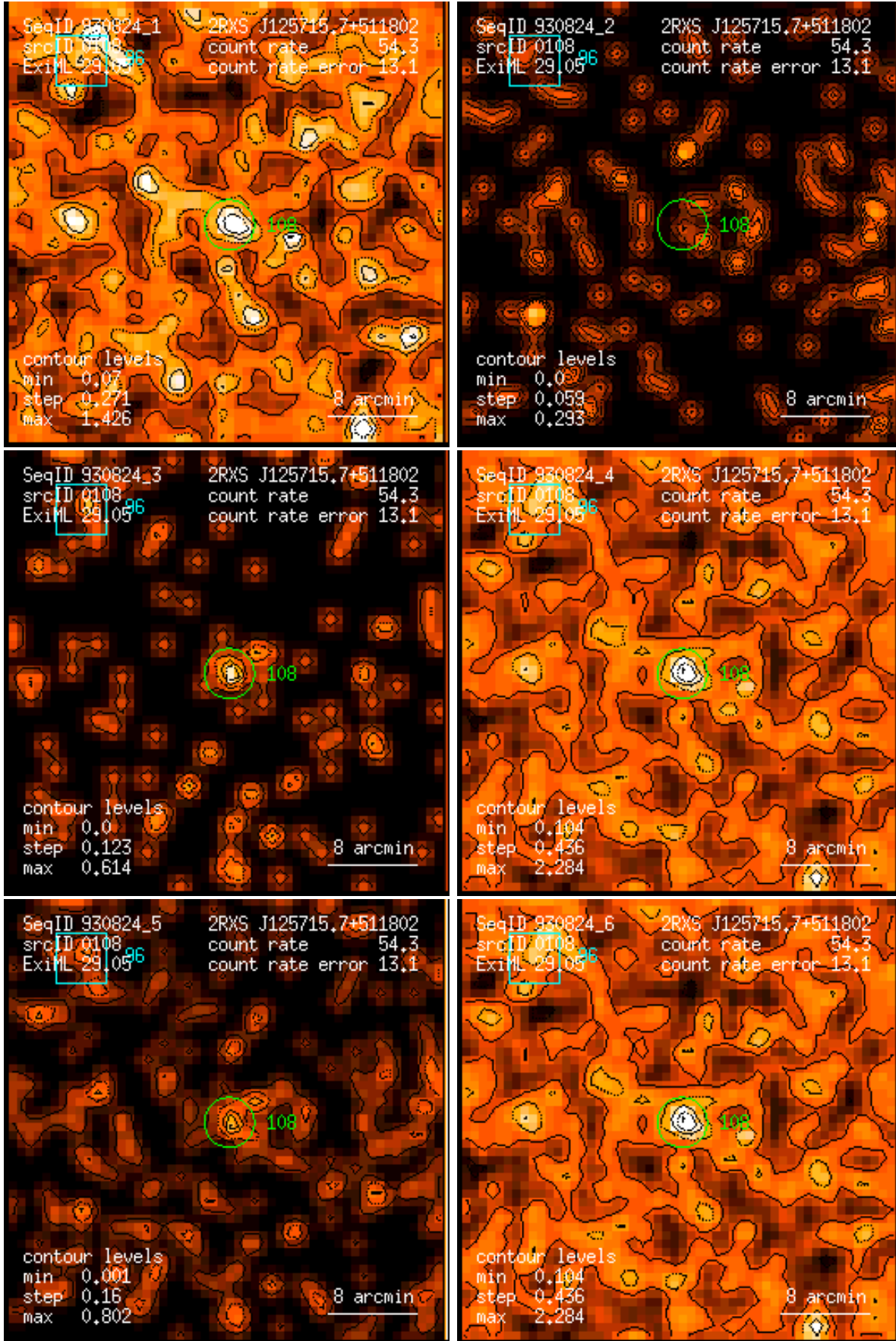
Figure 108: RASS 930824: detection 0108: band rate images, Gaussian filter: (1) PSPC channels 11 – 41, (2) 52 – 90, (3) 91 – 201, (4) 11 – 235, (5) 52 – 201, (6) 11 – 201. Broad band rates in counts/ks. Band rate contour levels in counts/ks/arcmin 2 .
