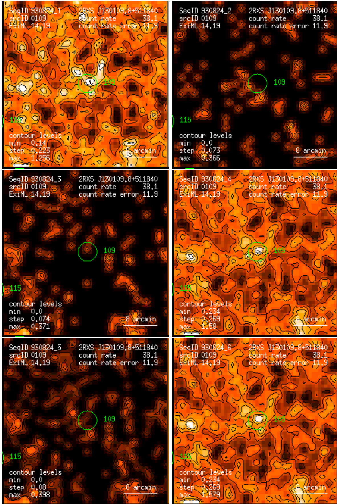
Figure 109: RASS 930824: detection 0109: band rate images, Gaussian filter: (1) PSPC channels 11 – 41, (2) 52 – 90, (3) 91 – 201, (4) 11 – 235, (5) 52 – 201, (6) 11 – 201. Broad band rates in counts/ks. Band rate contour levels in counts/ks/arcmin 2 .
