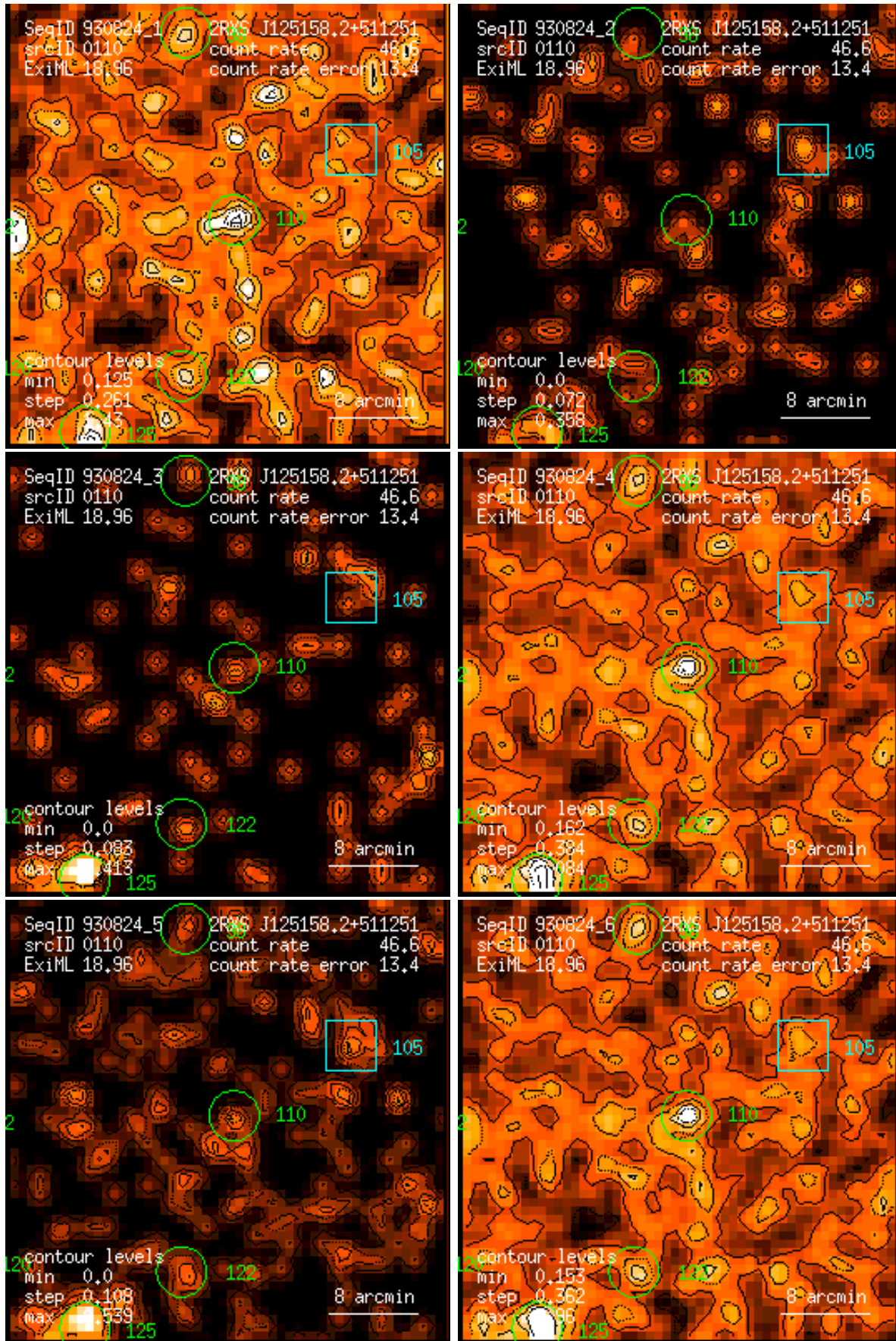
Figure 110: RASS 930824: detection 0110: band rate images, Gaussian filter: (1) PSPC channels 11 – 41, (2) 52 – 90, (3) 91 – 201, (4) 11 – 235, (5) 52 – 201, (6) 11 – 201. Broad band rates in counts/ks. Band rate contour levels in counts/ks/arcmin 2 .
