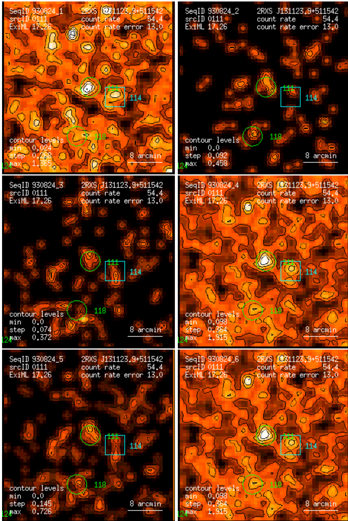
Figure 111: RASS 930824: detection 0111: band rate images, Gaussian filter: (1) PSPC channels 11 – 41, (2) 52 – 90, (3) 91 – 201, (4) 11 – 235, (5) 52 – 201, (6) 11 – 201. Broad band rates in counts/ks. Band rate contour levels in counts/ks/arcmin 2 .
