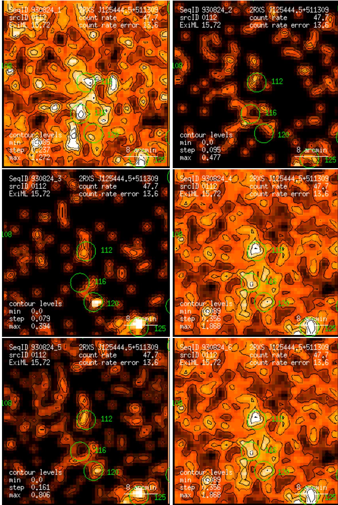
Figure 112: RASS 930824: detection 0112: band rate images, Gaussian filter: (1) PSPC channels 11 – 41, (2) 52 – 90, (3) 91 – 201, (4) 11 – 235, (5) 52 – 201, (6) 11 – 201. Broad band rates in counts/ks. Band rate contour levels in counts/ks/arcmin 2 .
