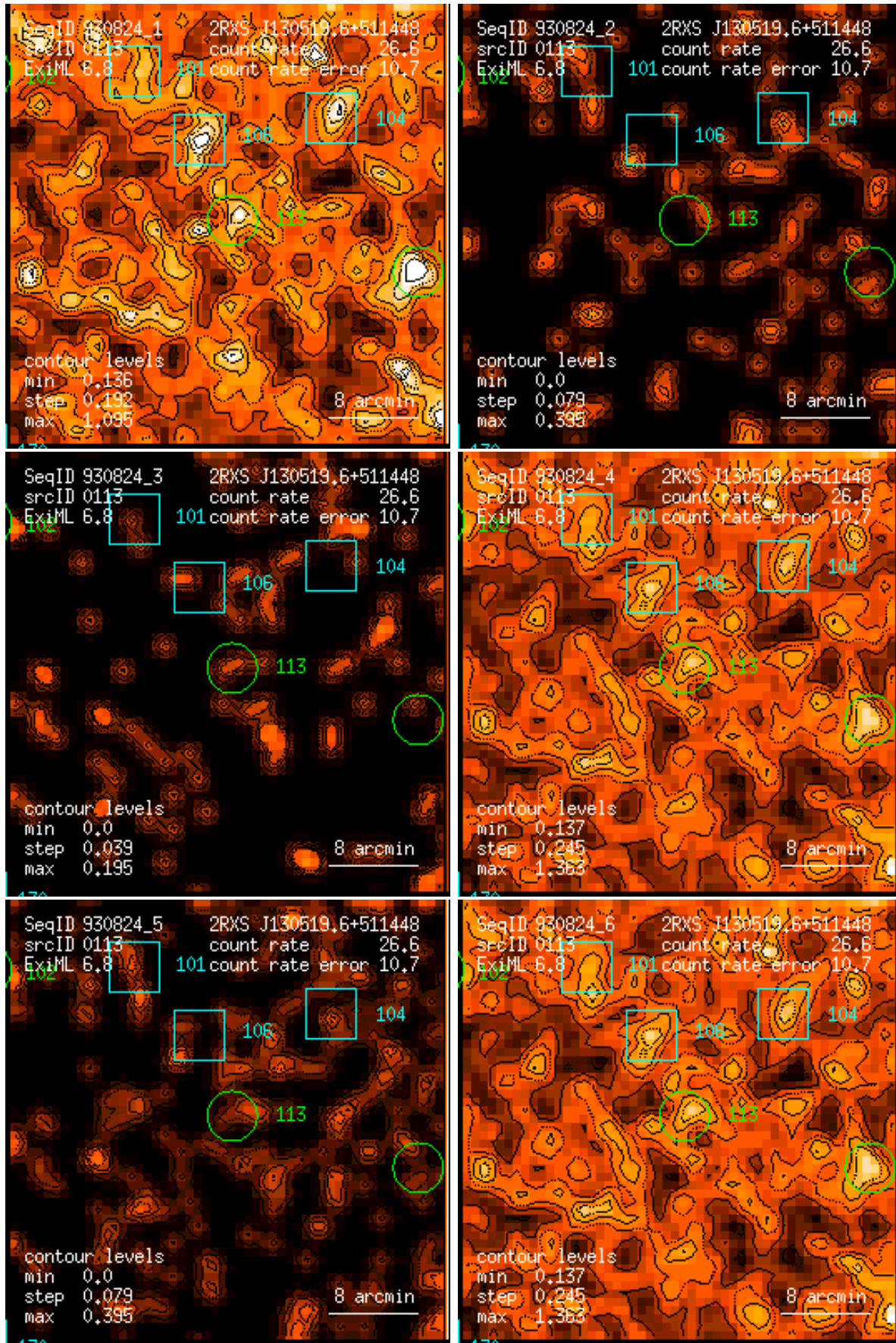
Figure 113: RASS 930824: detection 0113: band rate images, Gaussian filter: (1) PSPC channels 11 – 41, (2) 52 – 90, (3) 91 – 201, (4) 11 – 235, (5) 52 – 201, (6) 11 – 201. Broad band rates in counts/ks. Band rate contour levels in counts/ks/arcmin 2 .
