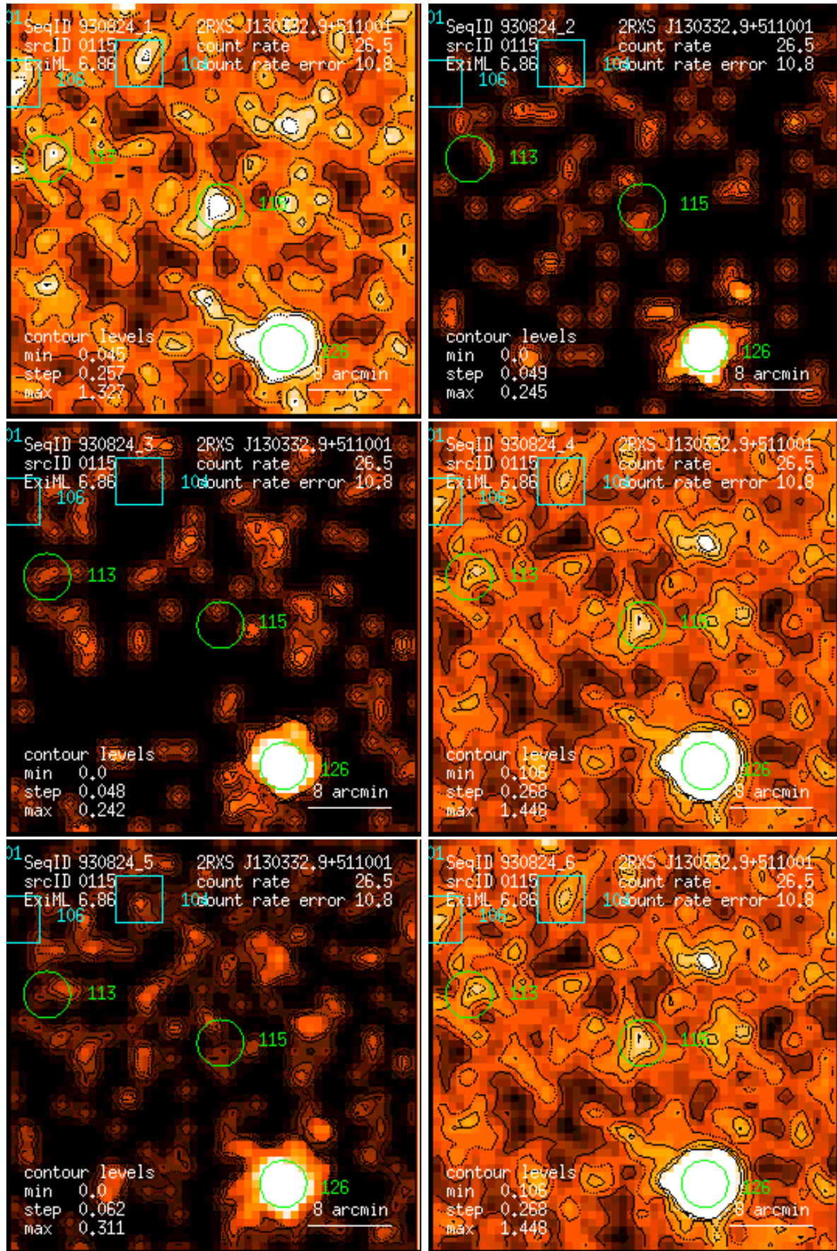
Figure 115: RASS 930824: detection 0115: band rate images, Gaussian filter: (1) PSPC channels 11 – 41, (2) 52 – 90, (3) 91 – 201, (4) 11 – 235, (5) 52 – 201, (6) 11 – 201. Broad band rates in counts/ks. Band rate contour levels in counts/ks/arcmin 2 .
